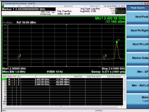
2402 MHz – Average
