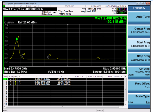
2480MHz – Average
