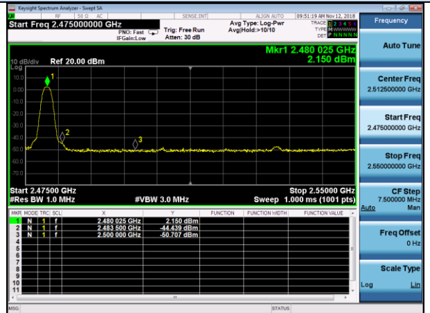
2480 MHz – Peak
