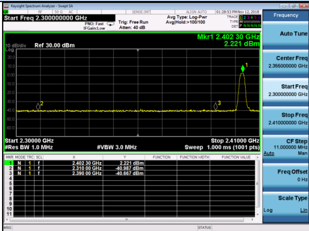
2402 MHz – Peak
