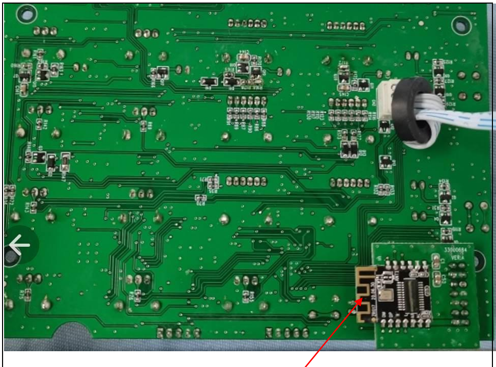
RF Antenna
