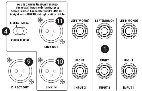
DA2112 REAR PANEL
