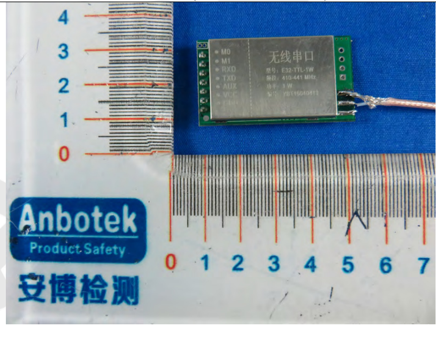
10. Figure PCB of the EUT-Front View (433.92MHz Module)
