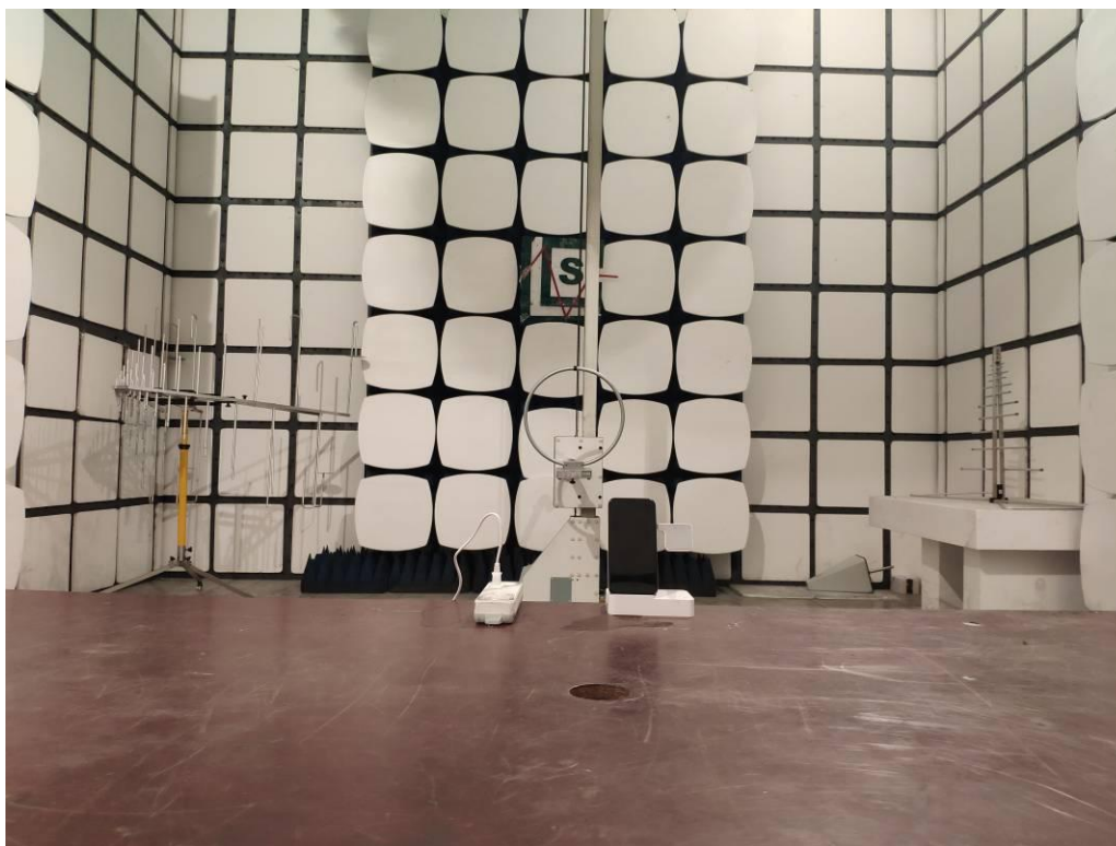
Radiated Emission below 30MHz-AC charge mode
