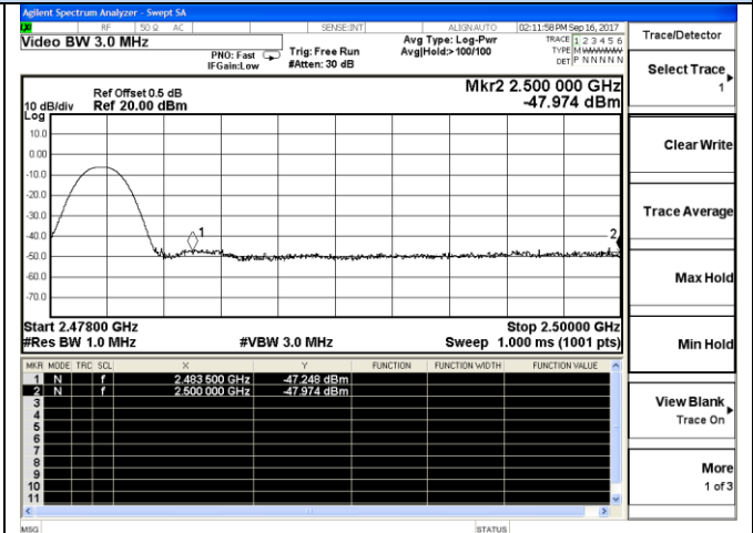
Channel 78 / 2480 MHz – Peak
