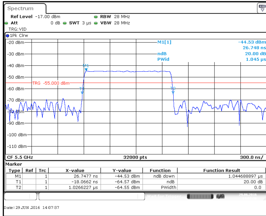
Radar Type 0 – single 1 μs pulse
