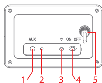
(Back panel)
