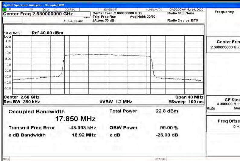
Band41-20MHz-16QAM-41490-100RB#0-17.850
