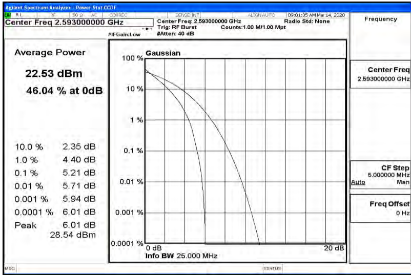
Band41-10MHz-QPSK-41540-1RB#0
