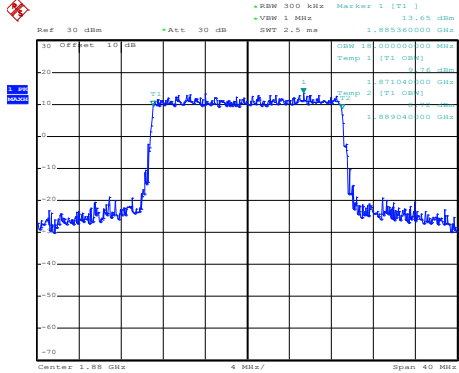
16QAM
