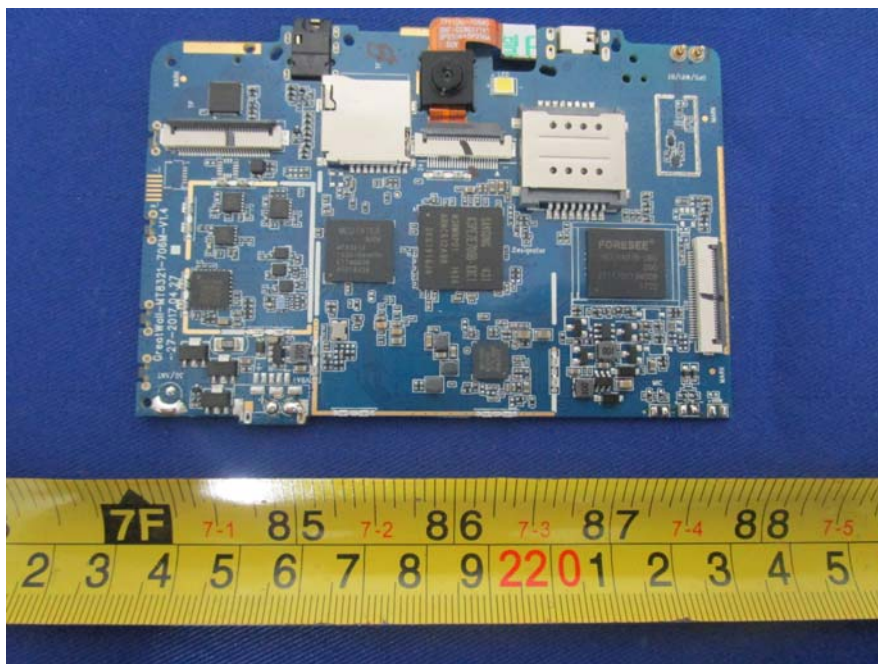
EUT – Main Board Top -8G Unshielded View
