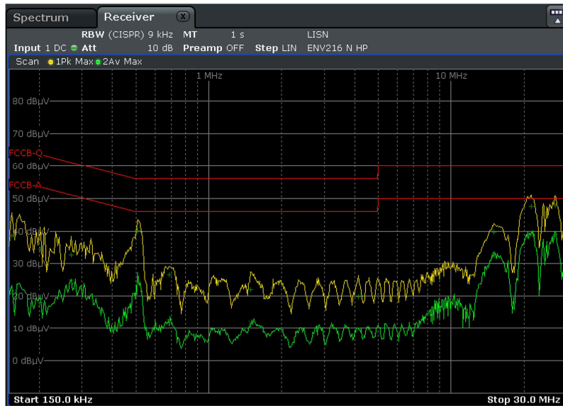
[Neutral line]
