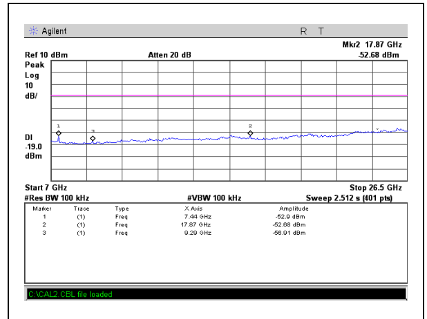
Highest Channel: 7 GHz ~ 26.5 GHz
