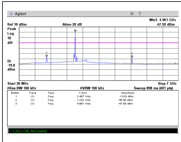
Highest Channel: 30 MHz ~ 7 GHz
