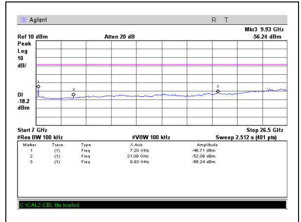
Middle Channel: 7 GHz ~ 26.5 GHz
