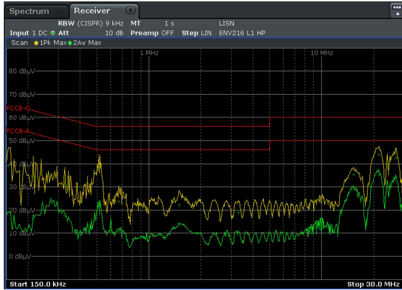
[Hot line]
