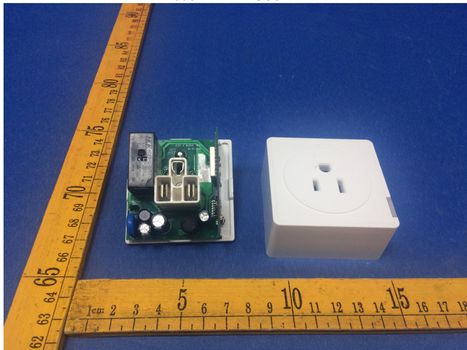
Model: HKWL-SO07WP
