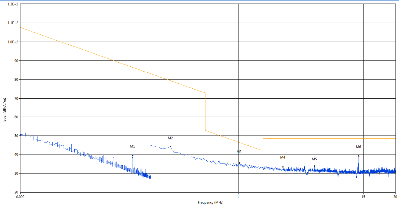
Below 30 MHz Horizontal
