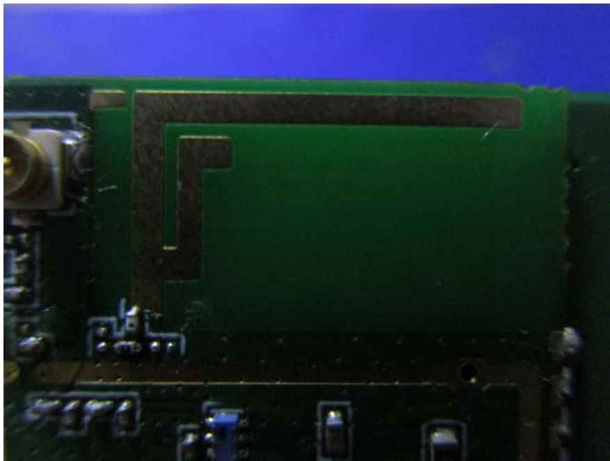
EUT-Antenna View
