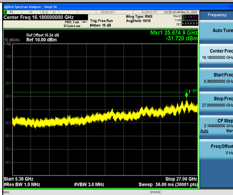
11AC20SISO-Ant1-5200-5360~27000-PASS
