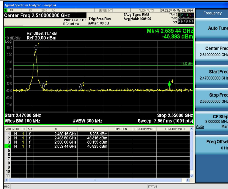
BLE_1M-Ant1-2480-PASS
