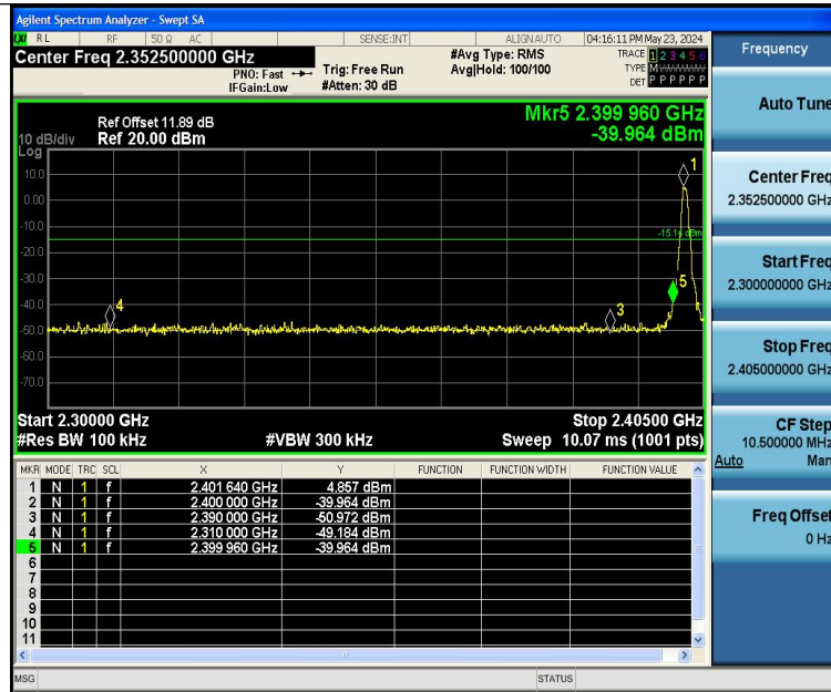
BLE_1M-Ant1-2402-PASS
