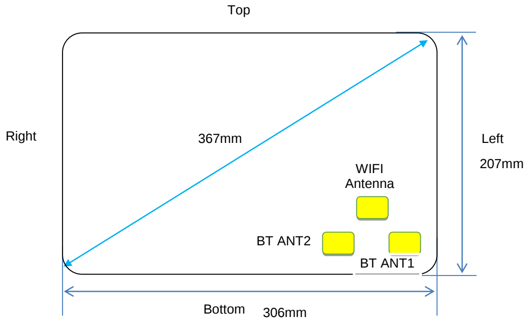
Keyboard Back View
