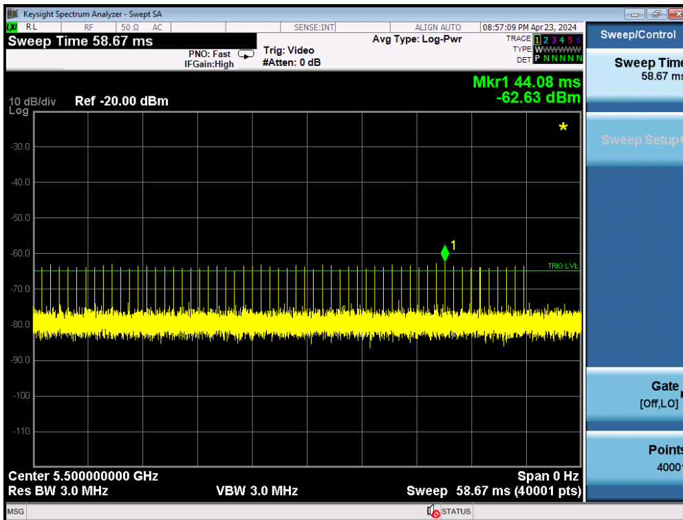
Radar Signal 1
