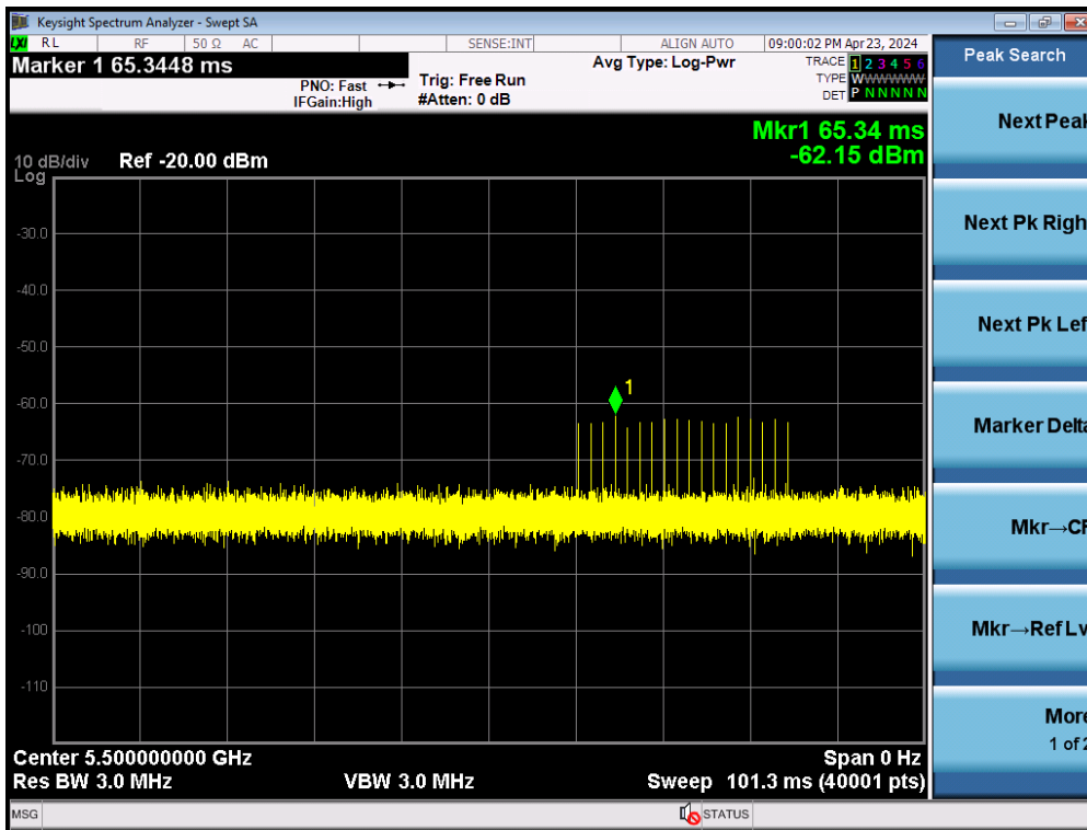
Radar Signal 1
