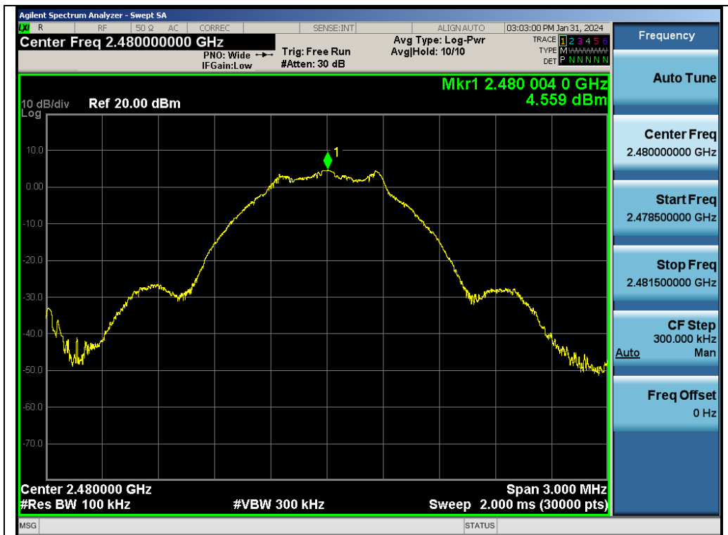
Test_Graph_LE2M_ANT1_2480_1Mbps_Reference Level
