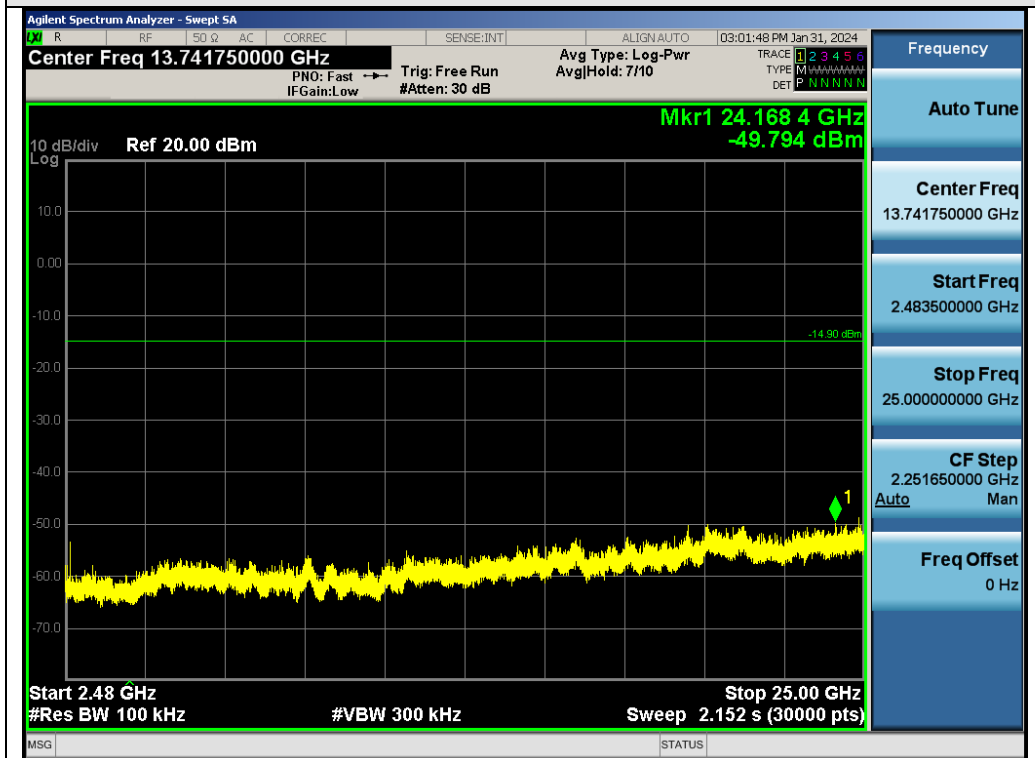
Test_Graph_LE2M_ANT1_2440_1Mbps_Higher Band Emissions
