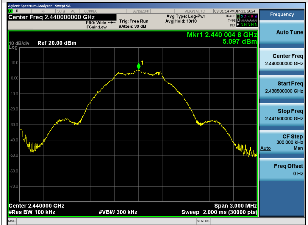
Test_Graph_LE2M_ANT1_2440_1Mbps_Reference Level
