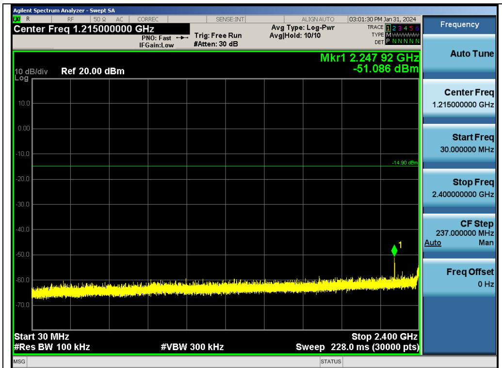
Test_Graph_LE2M_ANT1_2440_1Mbps_Lower Band Emissions
