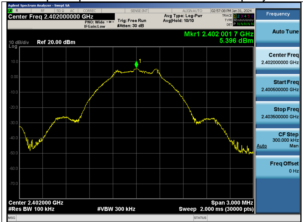
Test_Graph_LE2M_ANT1_2402_1Mbps_Reference Level
