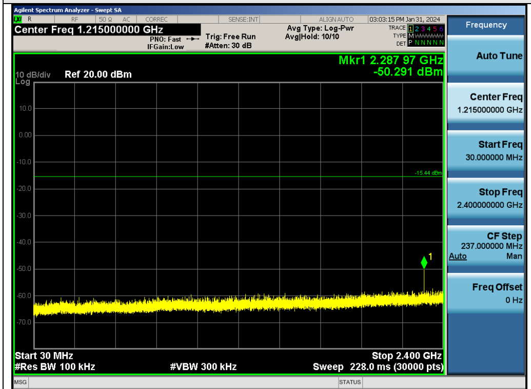
Test_Graph_LE2M_ANT1_2480_1Mbps_Lower Band Emissions
