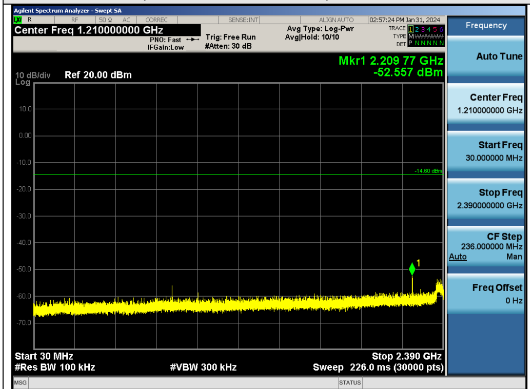
Test_Graph_LE2M_ANT1_2402_1Mbps_Lower Band Emissions
