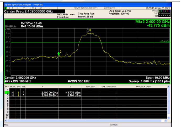
Out Of Band Emission π/4DQPSK_2-DH5_Channel 0
