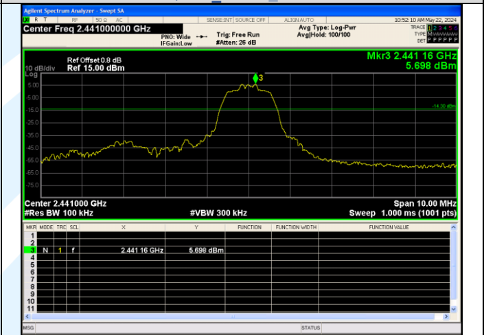
Out Of Band Emission \pi/4 QPSK_2-DH5_Channel 39
