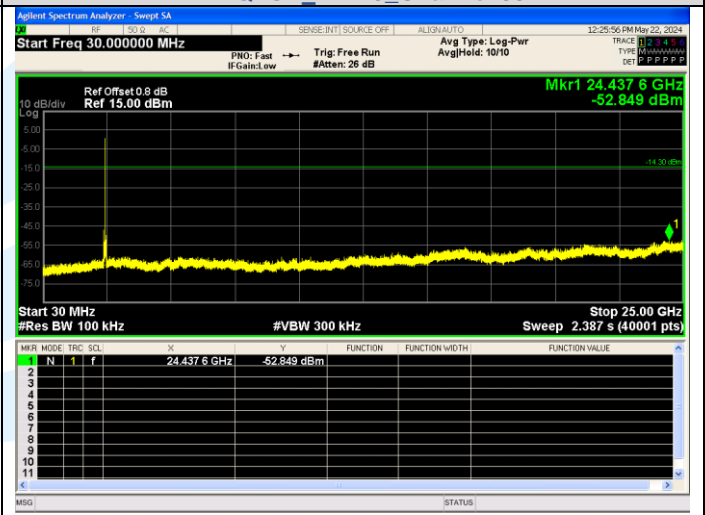
30.0 MHz - 25000.0 MHz \pi/4 QPSK_2-DH5_Channel 39
