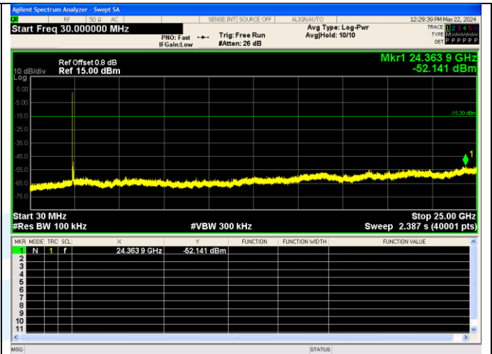
30.0 MHz - 25000.0 MHz \pi/4 QPSK_2-DH5_Channel 0
