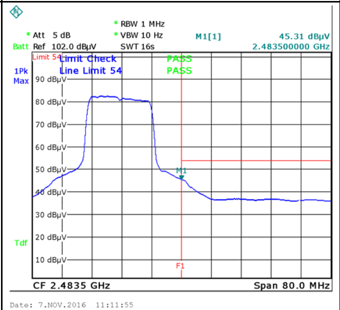
Band Edge, Right Side (Average) - 802.11g Note: F1 is frequency 2483.5MHz
