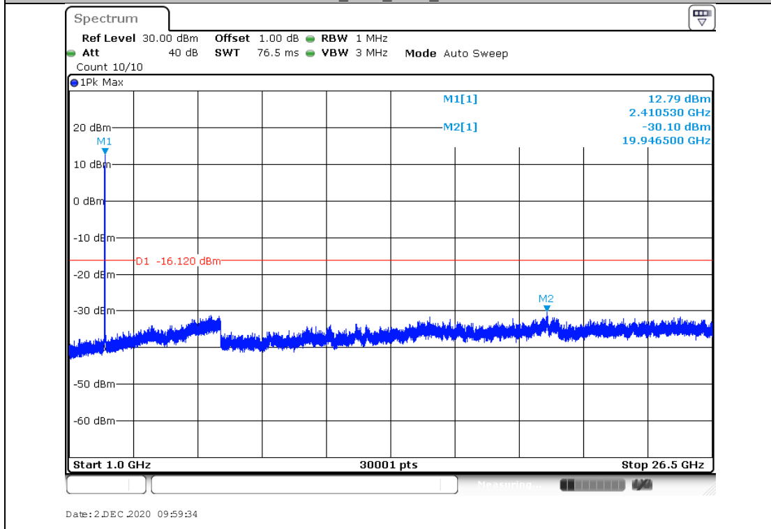
11N20SISO_Ant2_2412_0~Reference
