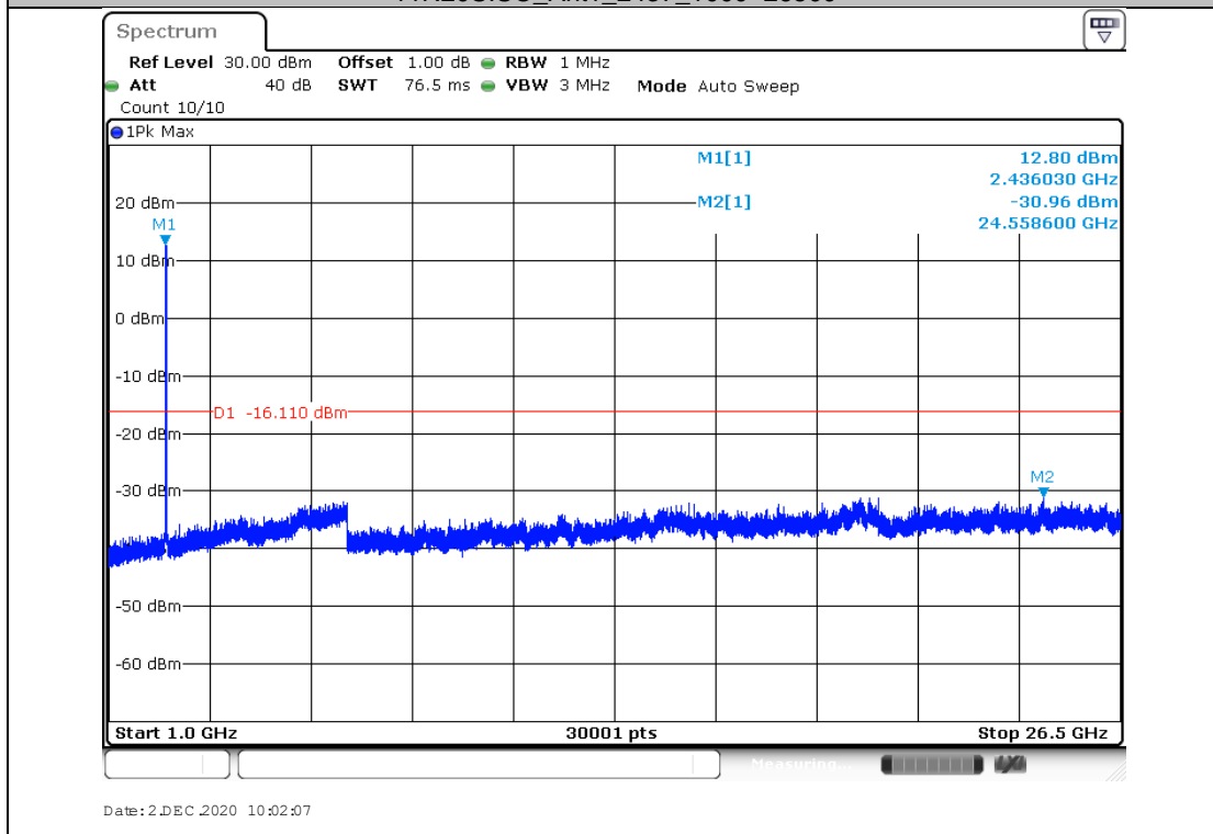
11N20SISO_Ant2_2437_0~Reference
