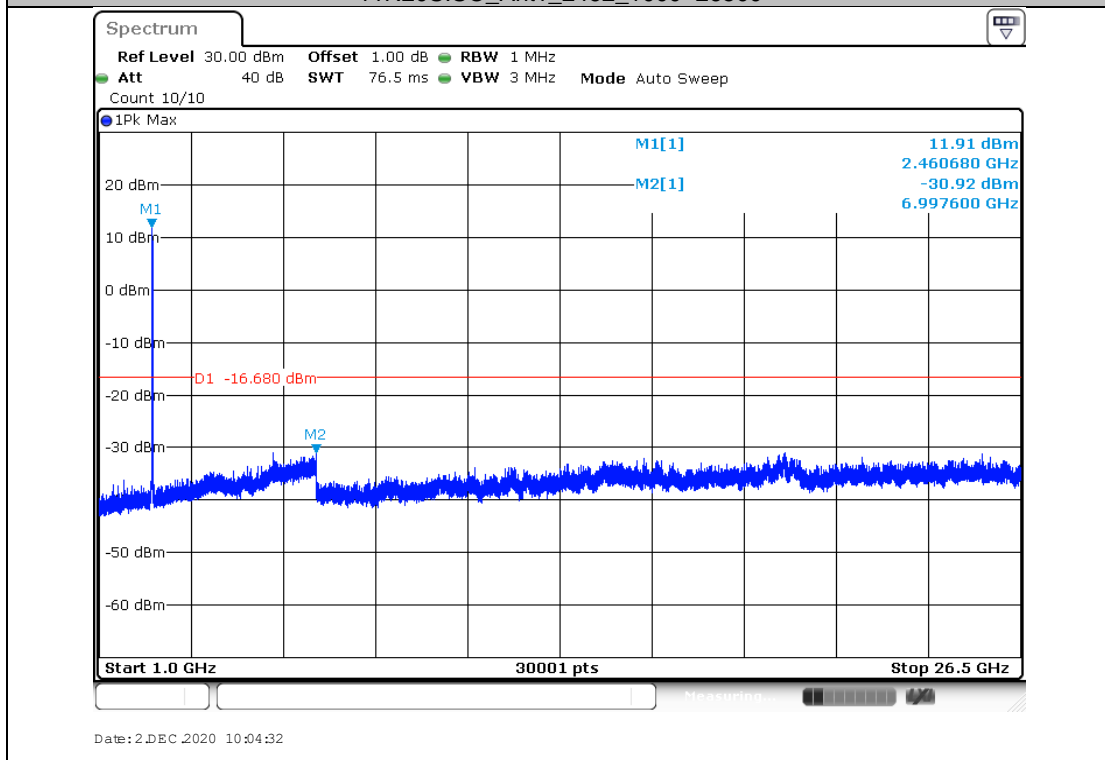
11N20SISO_Ant2_2462_0~Reference
