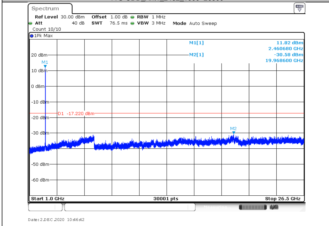
11G-CDD_Ant2_2462_0~Reference
