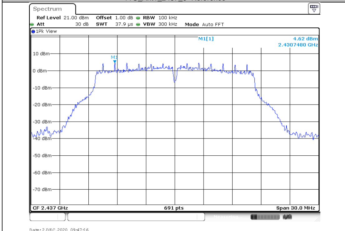
11G_Ant1_2437_0-Reference
