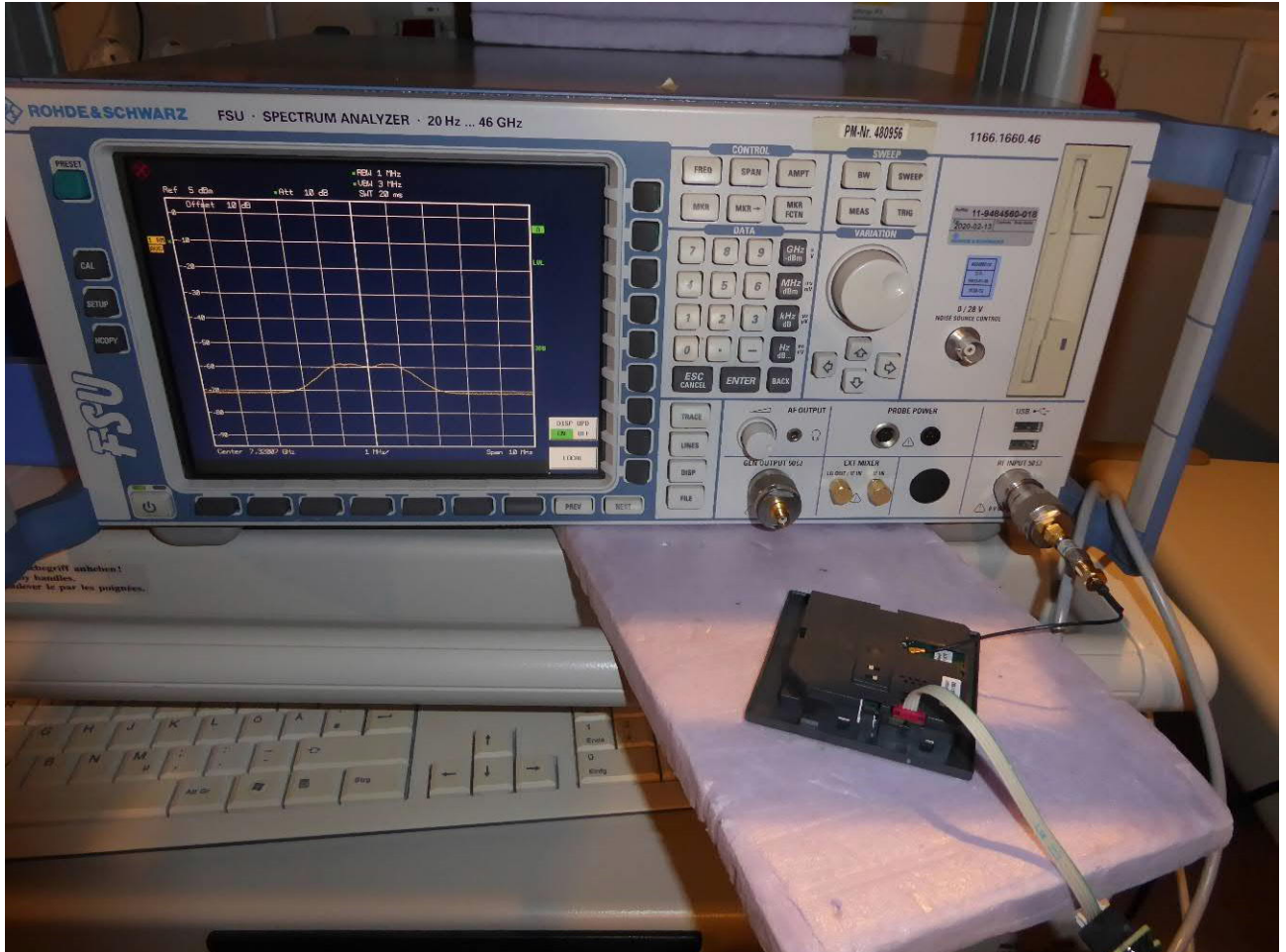
Test setup A406 – measurement at the antenna port
