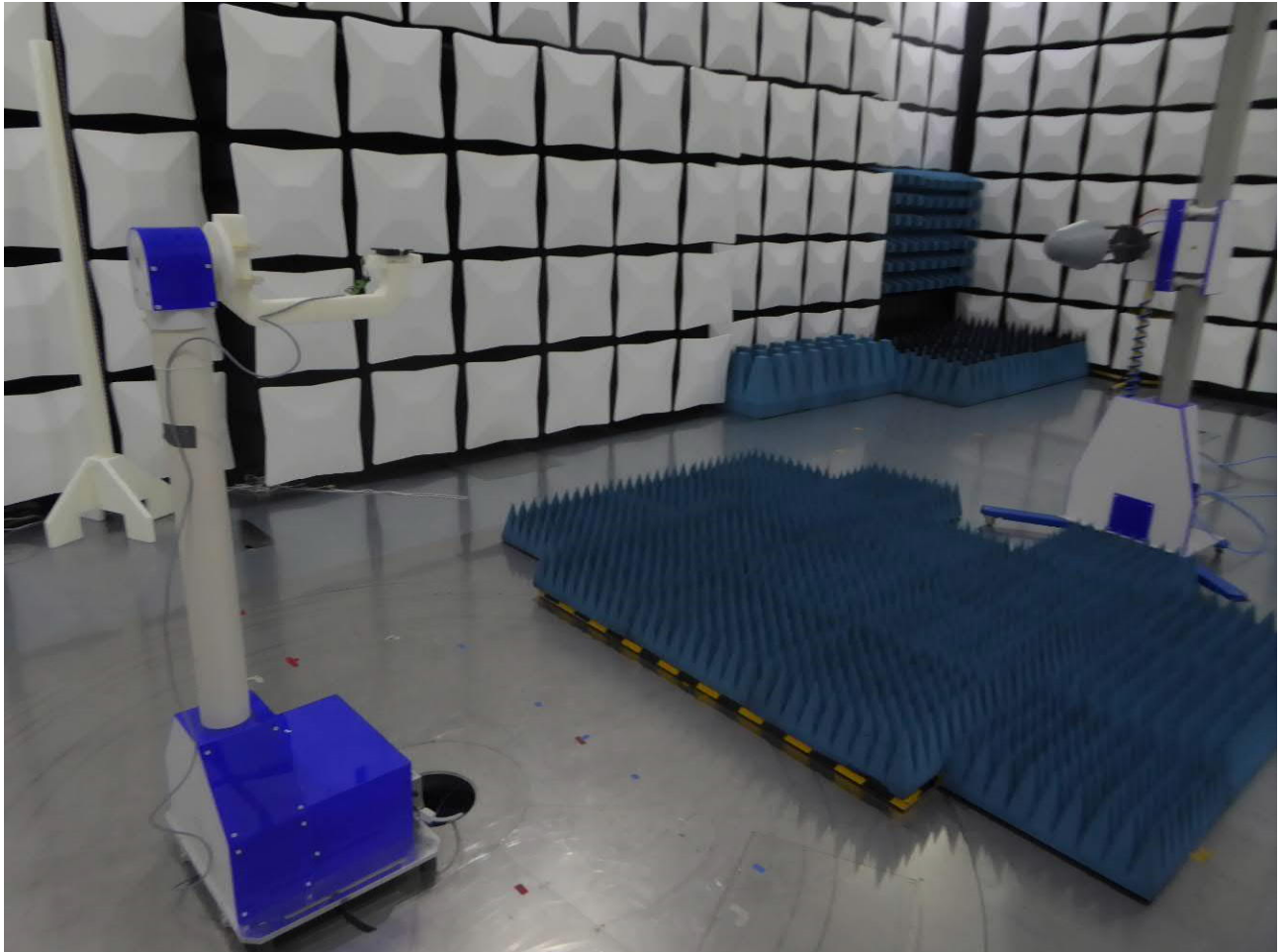
Test setup A406 – radiated test in semi-anechoic chamber with ground plane (M276)
