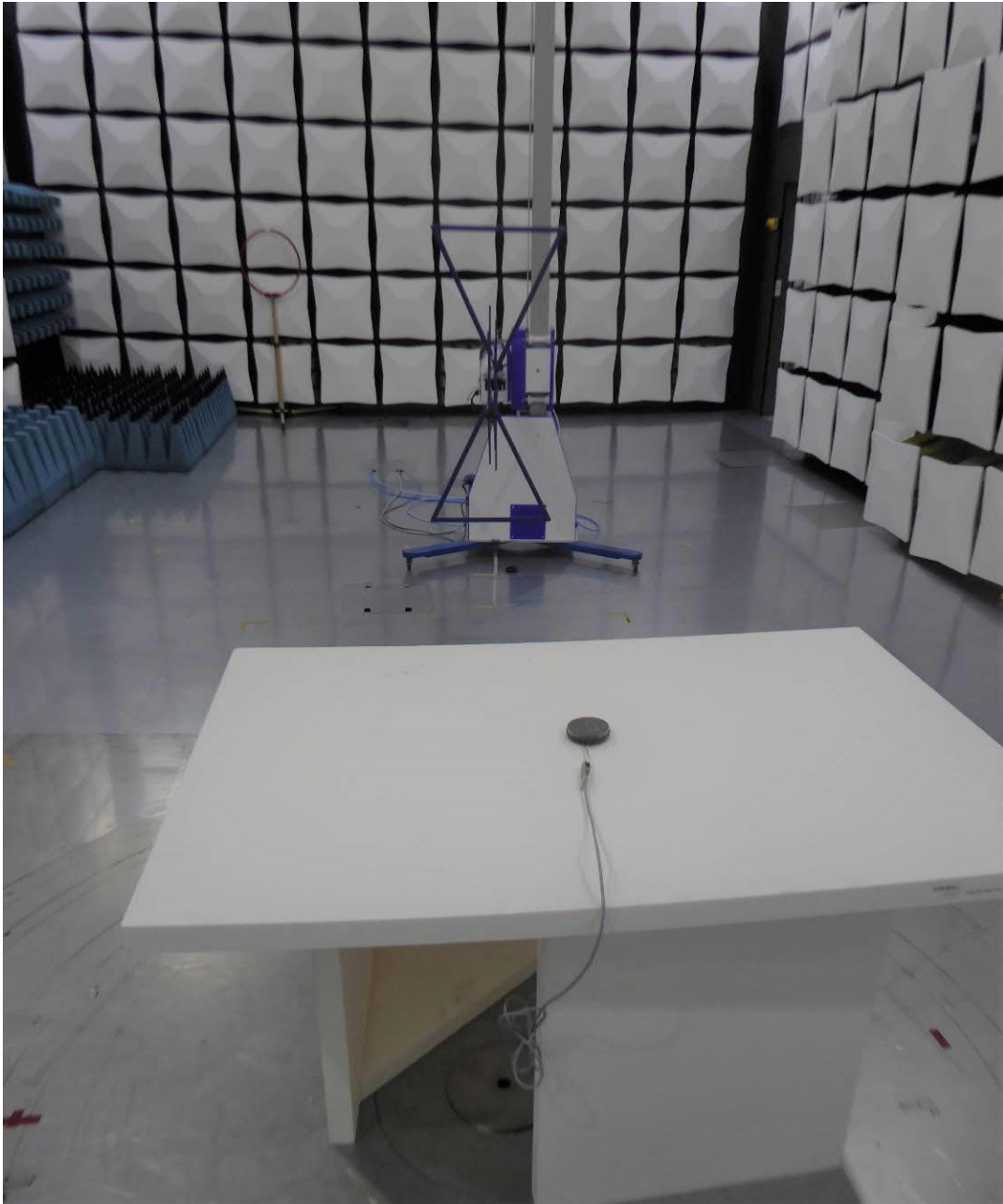
Test setup A400 – radiated test in semi-anechoic chamber (M276)
