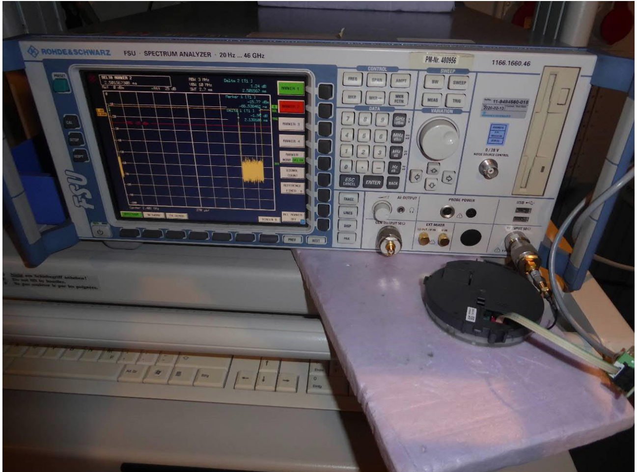
Test setup A400 – measurement at the antenna port
