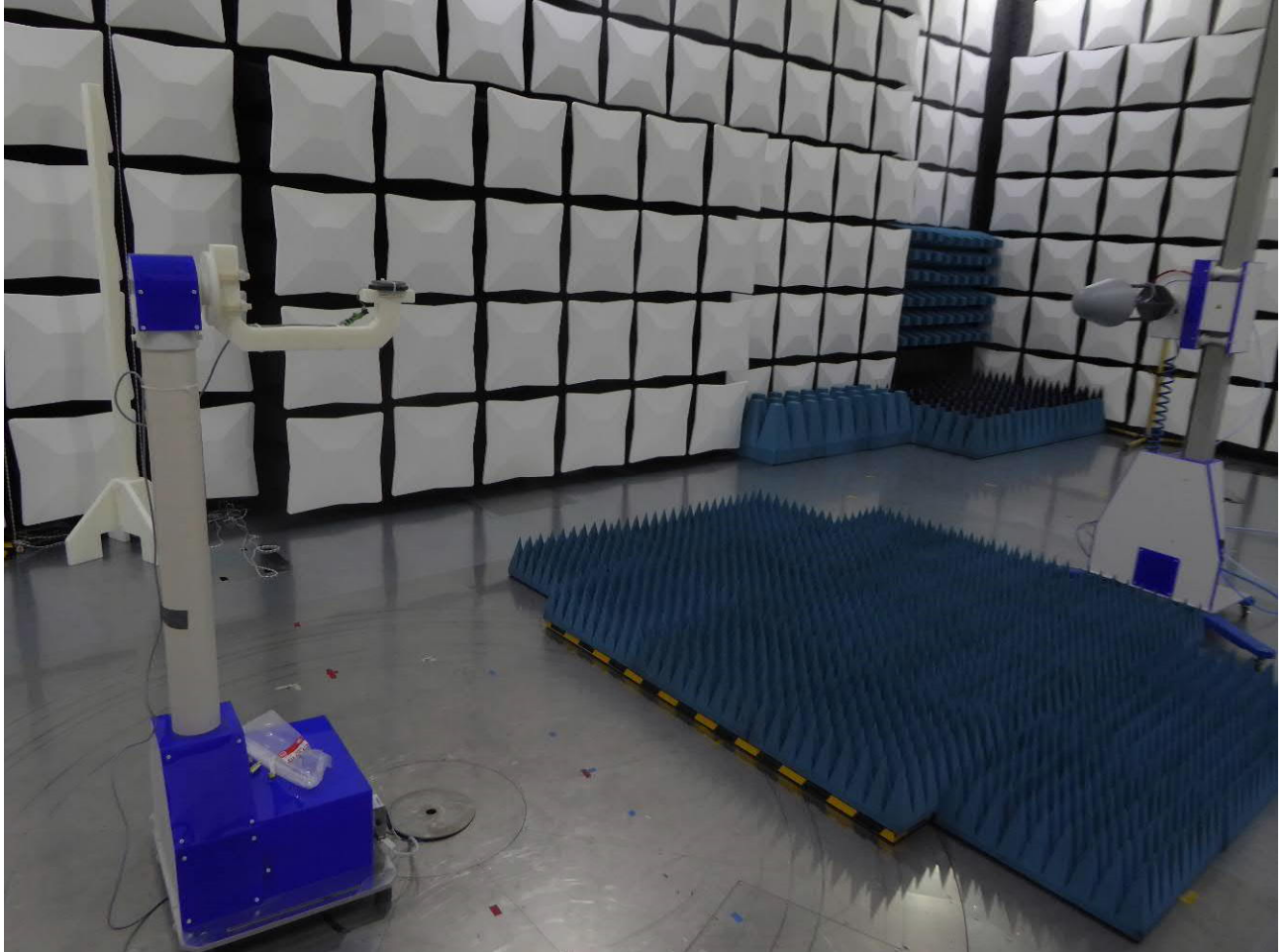
Test setup A400 – radiated test in semi-anechoic chamber with ground plane (M276)
