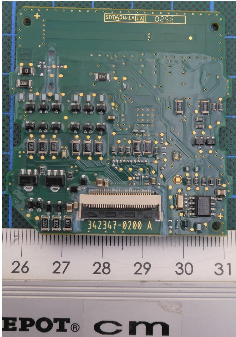
EUT A400 – Main PCB bottom view
