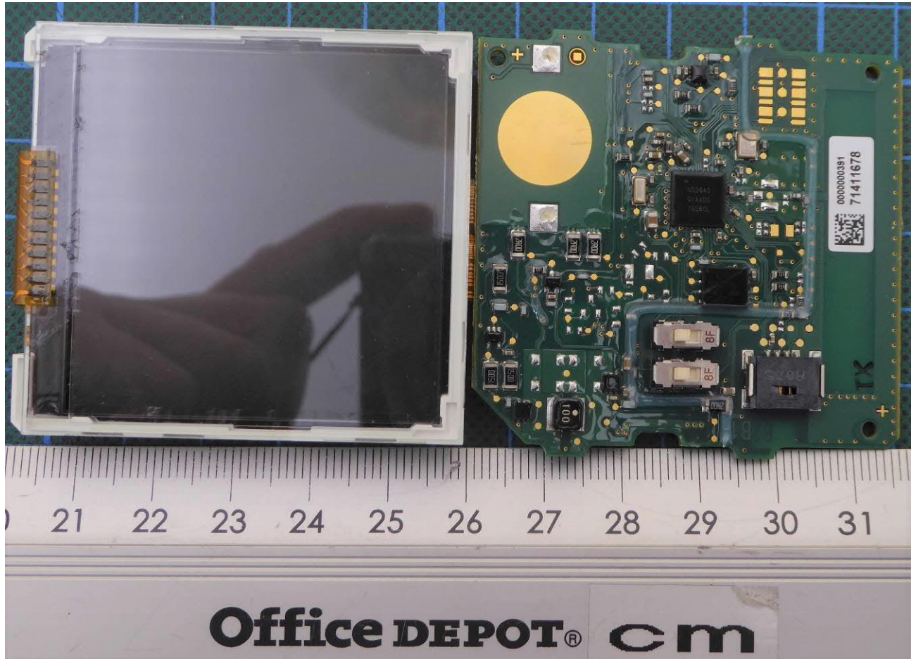
EUT A406 – internal view 4
