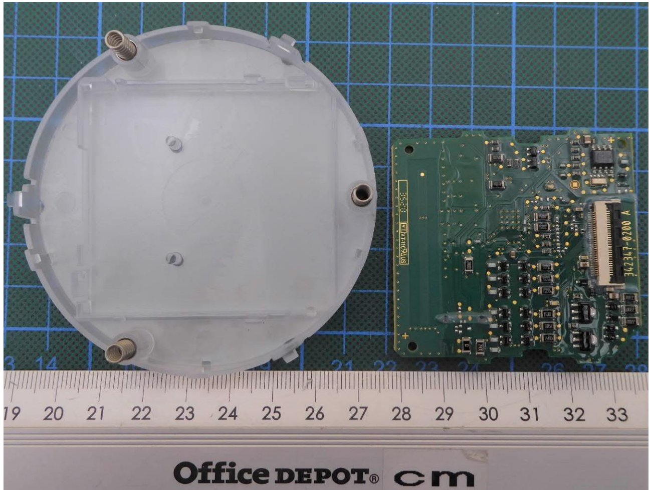
EUT A400 – internal view 2
