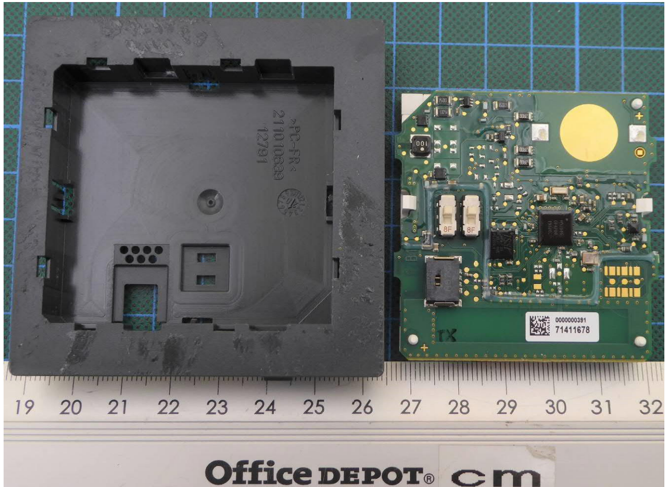
EUT A406 – internal view 2
