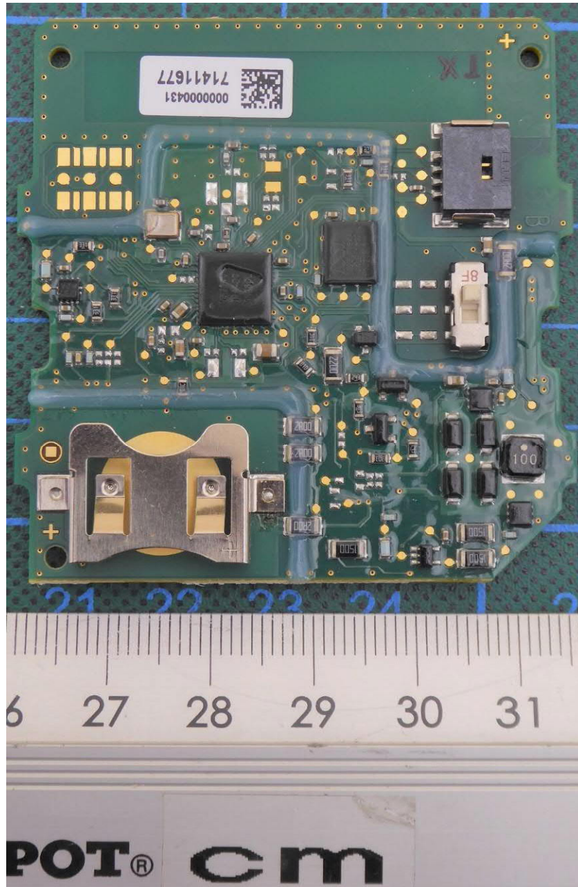
EUT A400 – Main PCB top view
