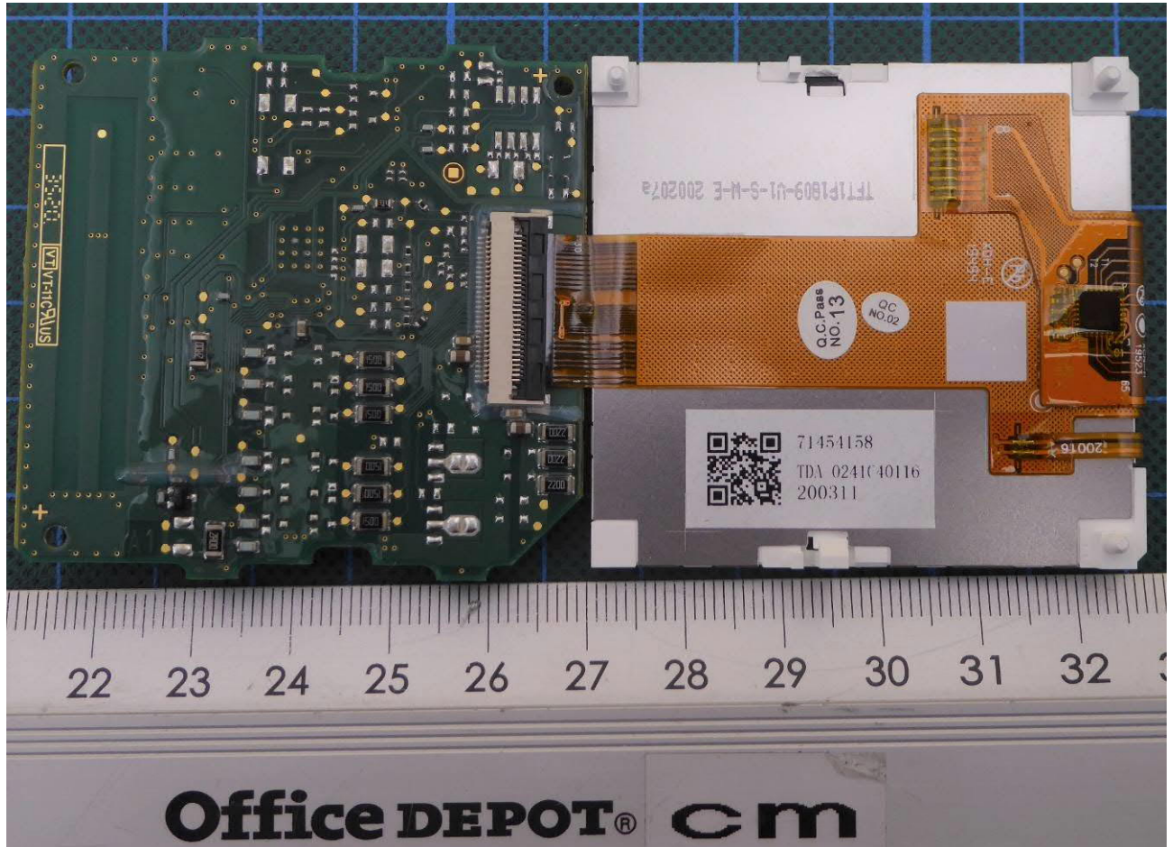
EUT A406 – internal view 3
