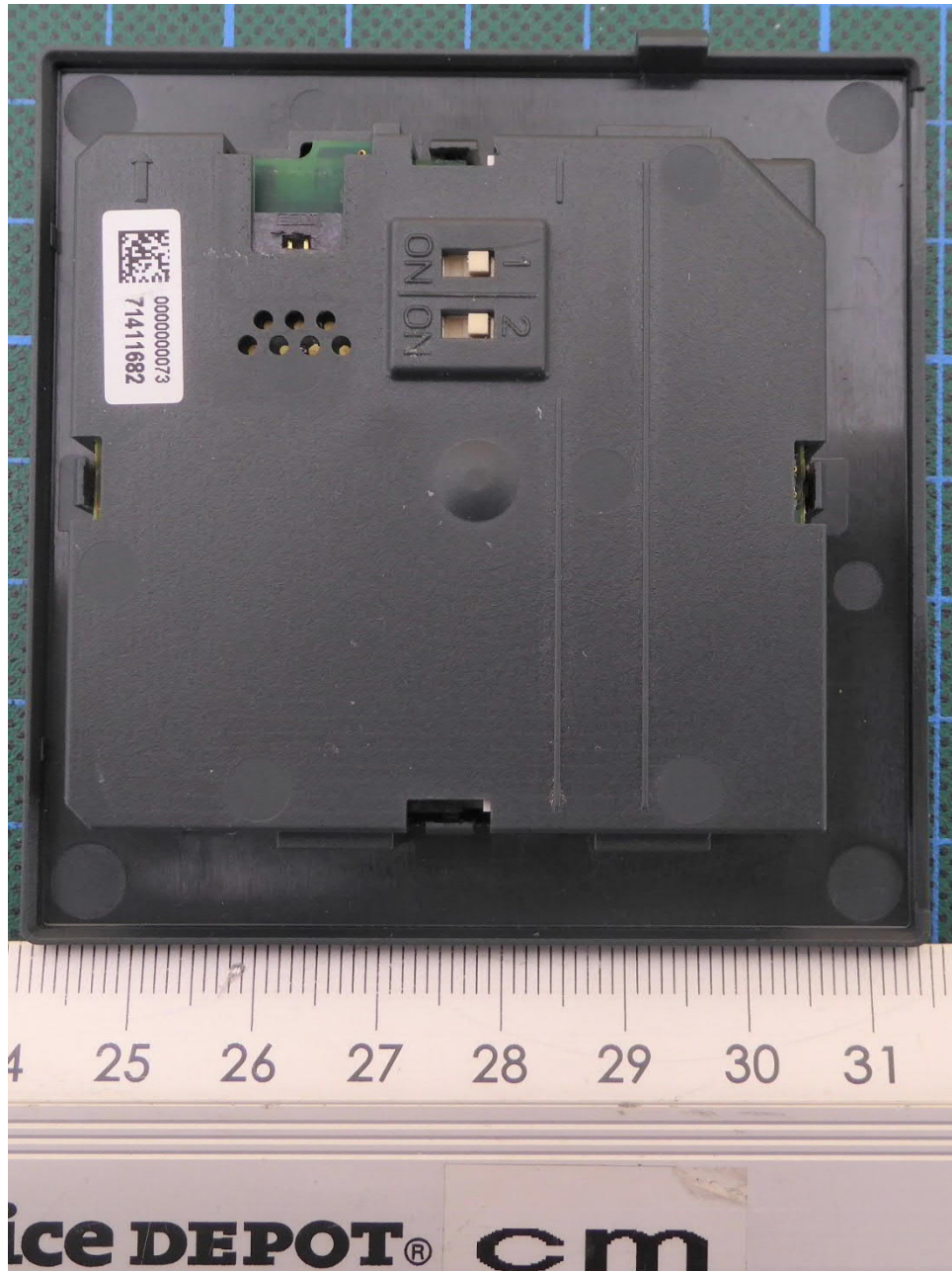
EUT A406 – bottom view with ribbon cable
