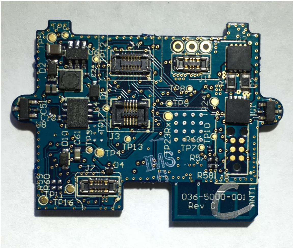
Figure 2: Photo of Main PCB - Top
