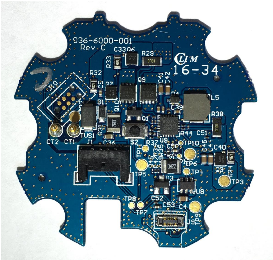
Figure 4: Photo of Charger PCB - Top
