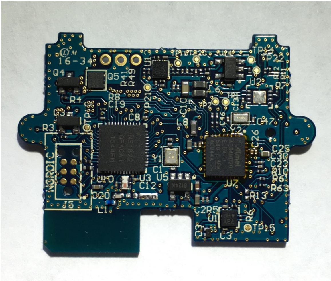
Figure 3: Photo Main PCB - Bottom
