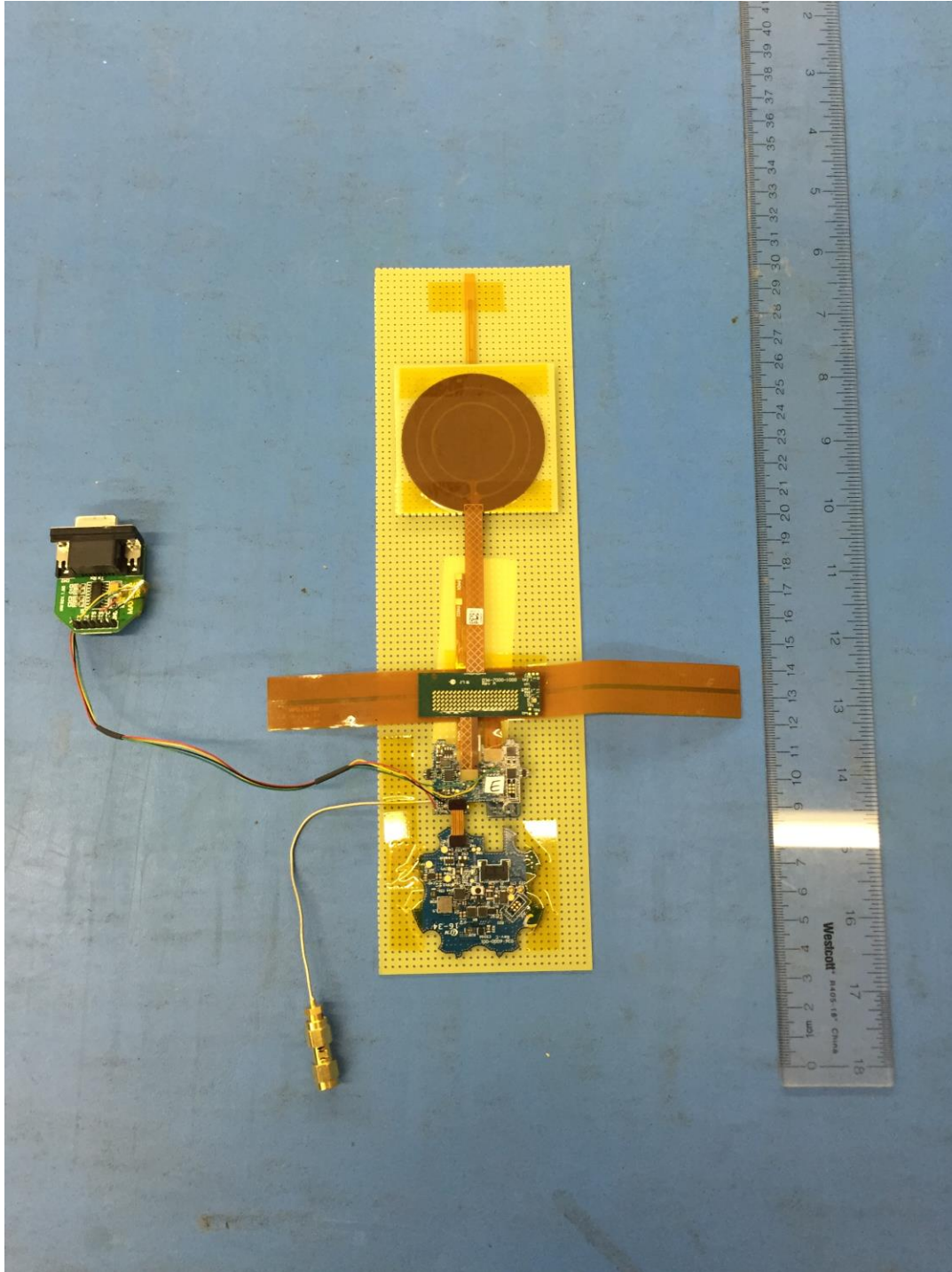
Figure 1: Photo of Conducted Test Sample - PCB (Top view)
