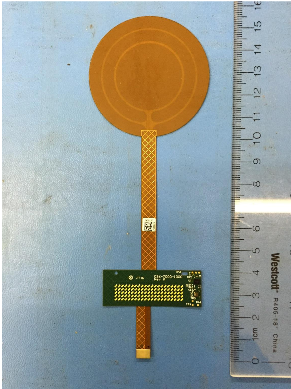
Figure 6: Photo of FPC1 – Top
