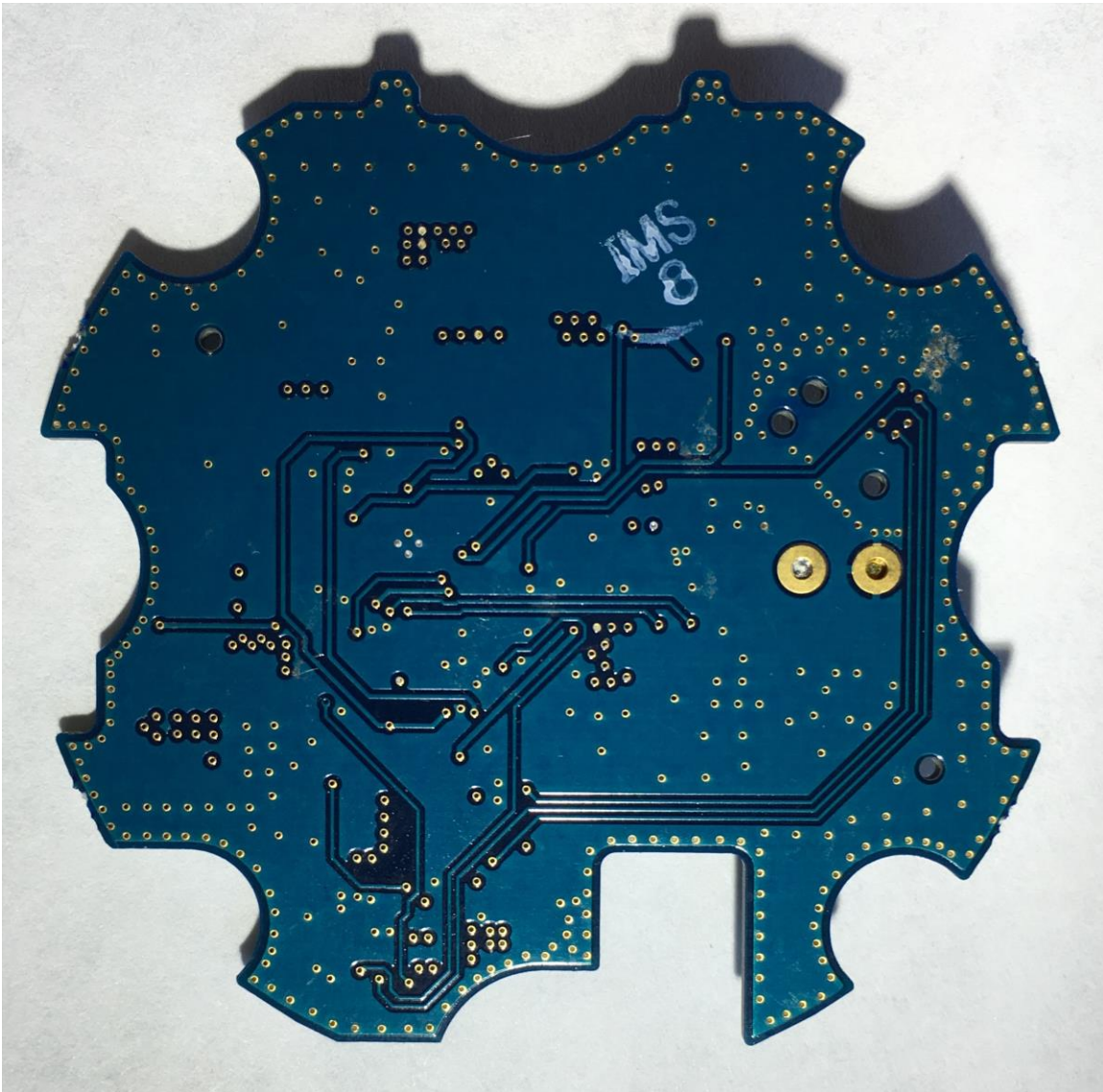
Figure 5: Photo of Charger PCB - Bottom
