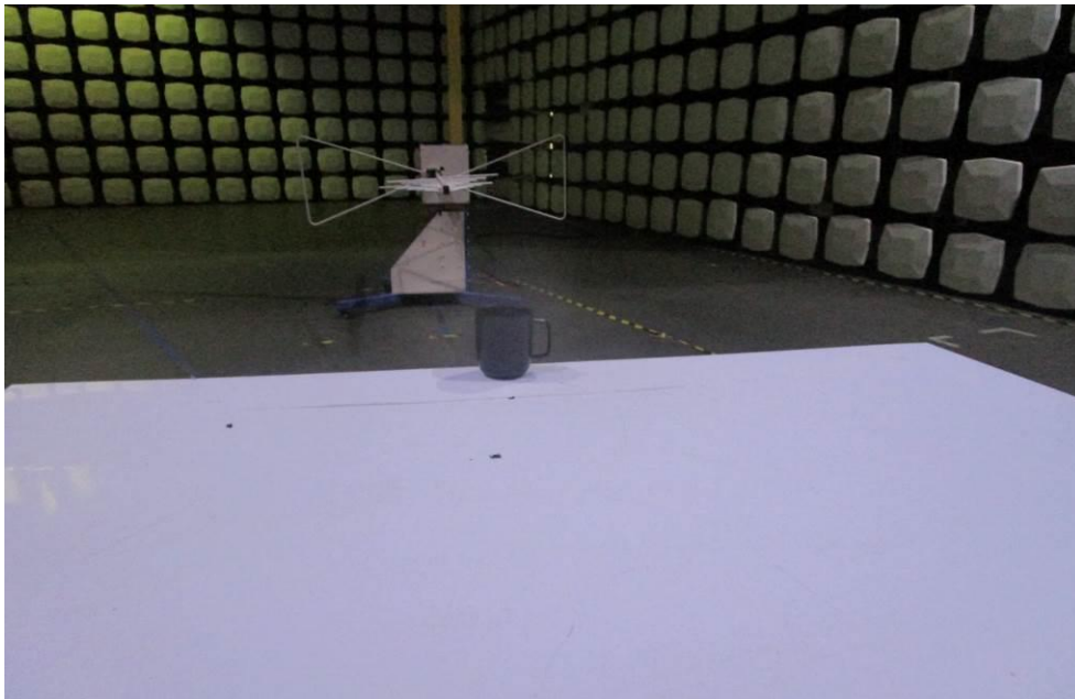
Radiated Spurious Emissions (Below 1GHz)
