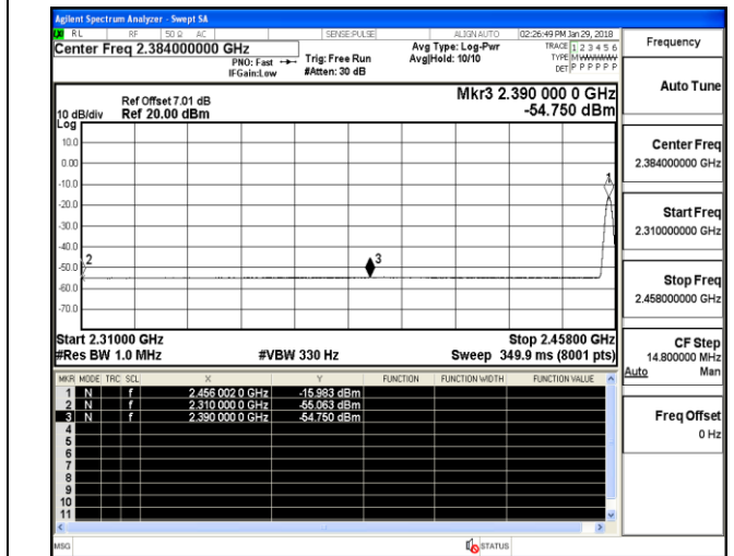
Channel 1 / 2456 MHz – Average
