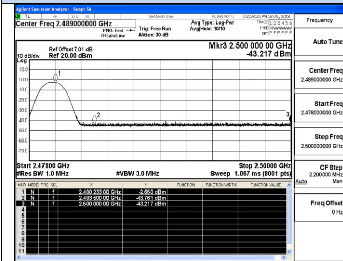
Channel 13 / 2480 MHz – Peak
