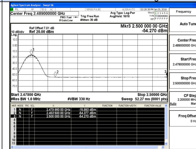
Channel 13 / 2480 MHz – Average
