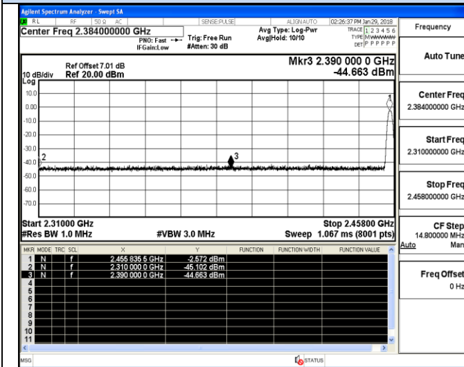
Channel 1 / 2456 MHz – Peak
