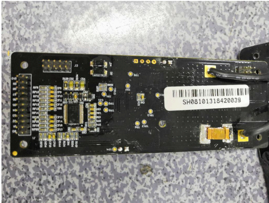
MAIN BOARD TOP VIEW (CLOSE-UP 2)
