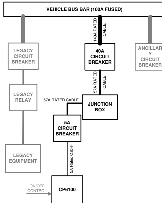
Figure 8: Typical Bus Power Supply Circuit Breaker and Cable Rating
