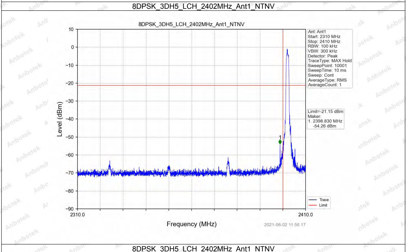
8DPSK_3DH5_LCH_2402MHz_Ant1_NTNV
