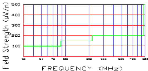
Figure 6-7. 3-Meter Limits
