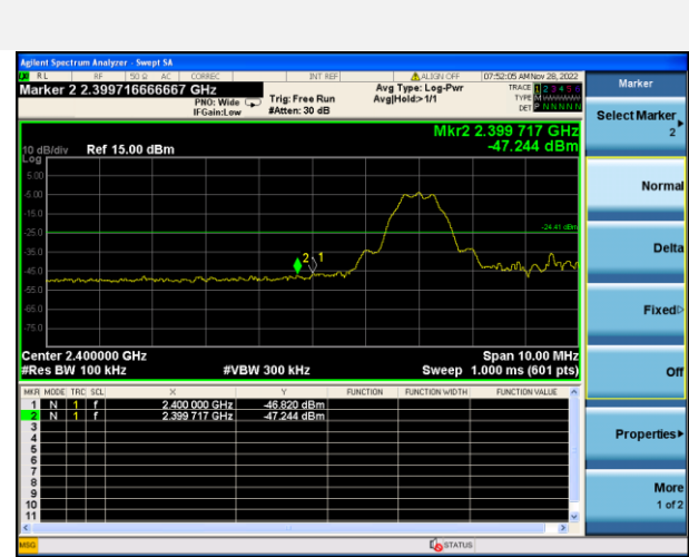
GFSK (BLE 1Mbps) LOW CHANNEL, BAND EDGE
