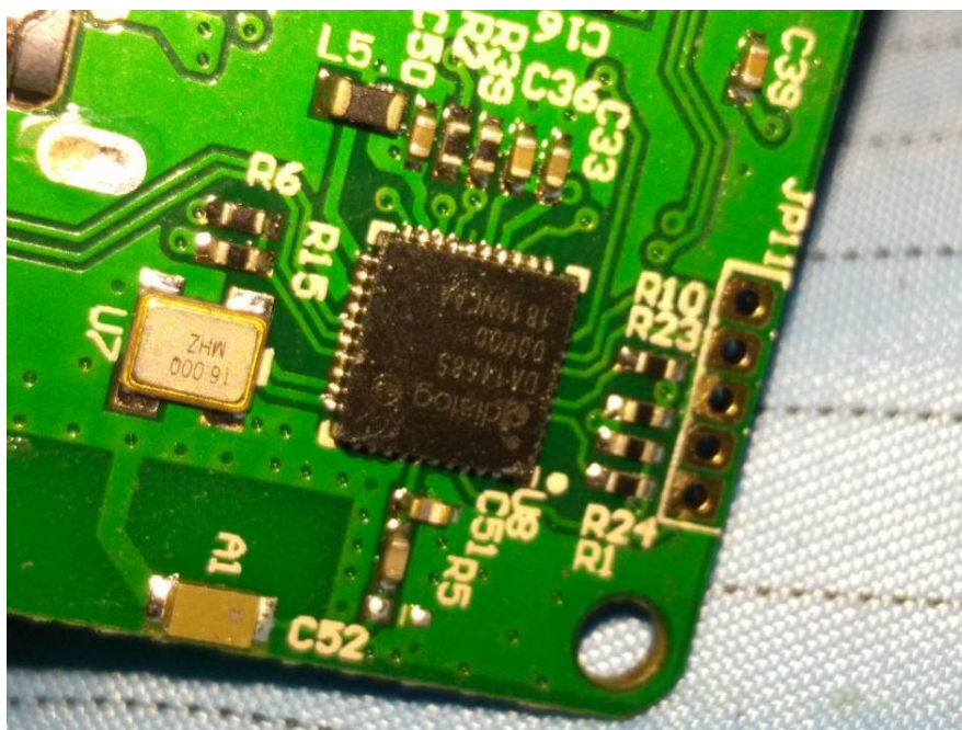
EUT – Bluetooth Board IC Chip View
