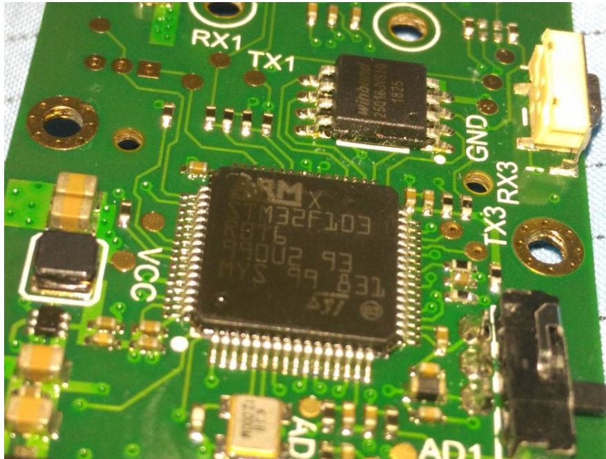
EUT – Small Board 2 IC Chip View
