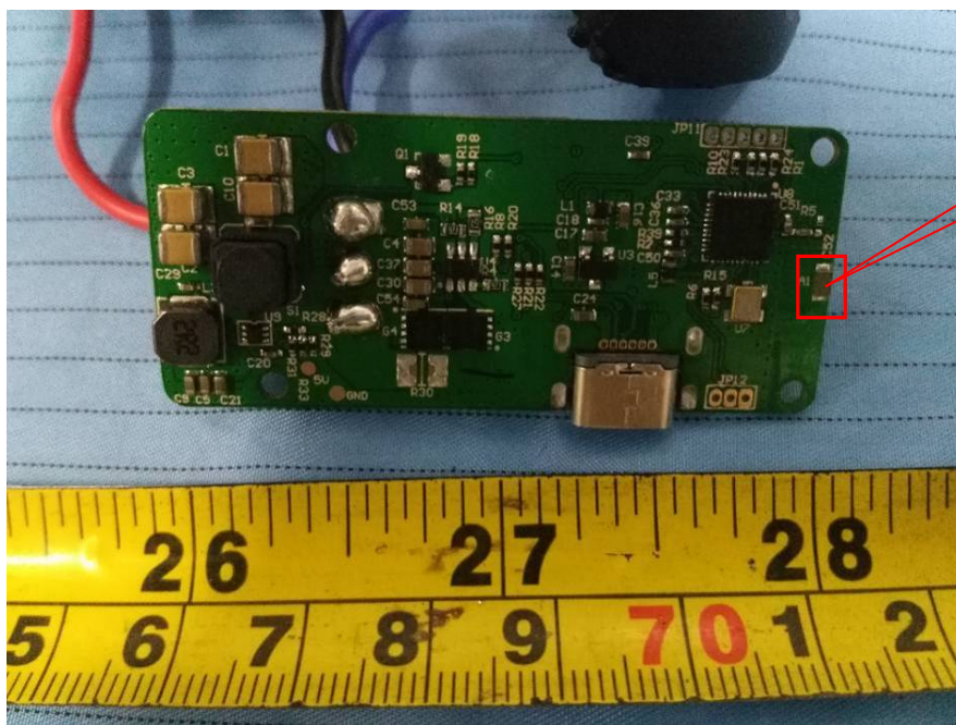
EUT – Bluetooth Main Board Top View
