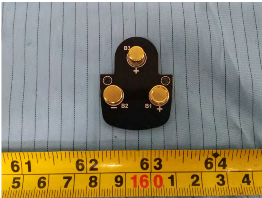
EUT – Small Board 2 Cover off View
