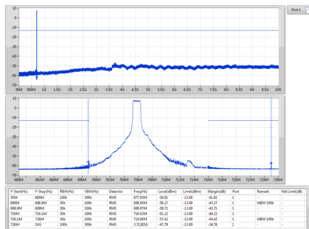
Band 12 LTE-M1_5MHz_Nss1_1TX 707.5MHz_16QAM_RB 6,#RB 0,NB 0
