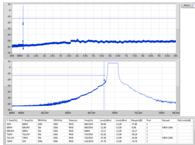
Band 12 LTE-M1_5MHz_Nss1_1TX 701.5MHz_16QAM_RB 1,#RB 0,NB 0
