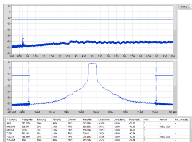
Band 12 LTE-M1_1.4MHz_Nss1_1TX 707.5MHz_QPSK_RB 6,#RB 0,NB 0
