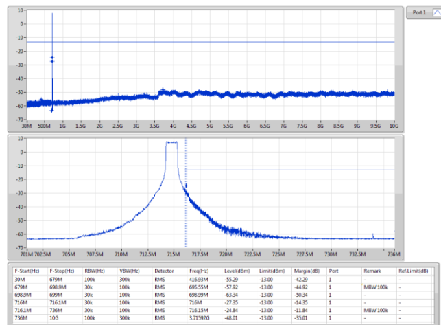
Band 12 LTE-M1_10MHz_Nss1_1TX 711MHz_16QAM_RB 1,#RB 5,NB 7
