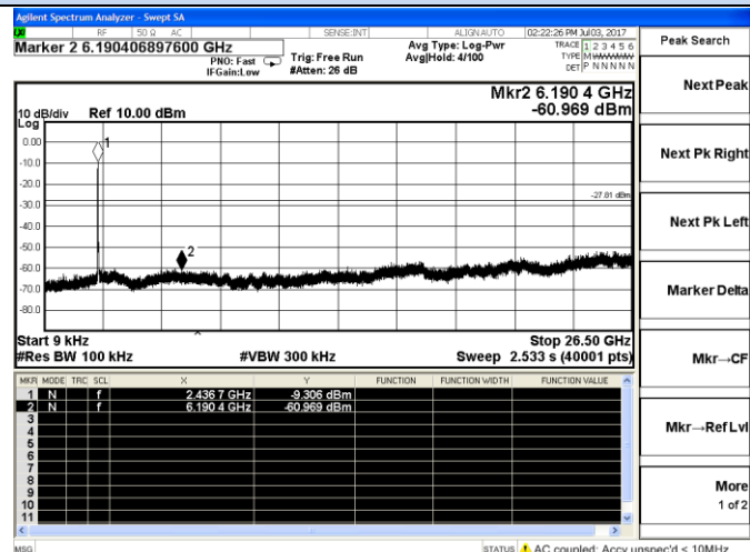
802.11n-HT40 Low channel
