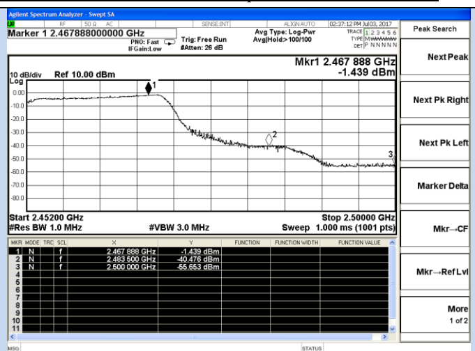
Channel 11 / 2452 MHz – Peak
