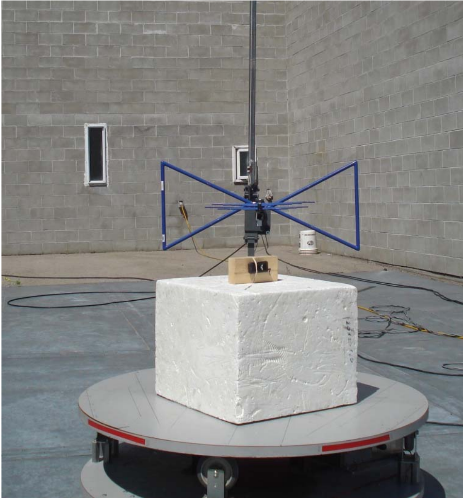
Radiated Emissions
