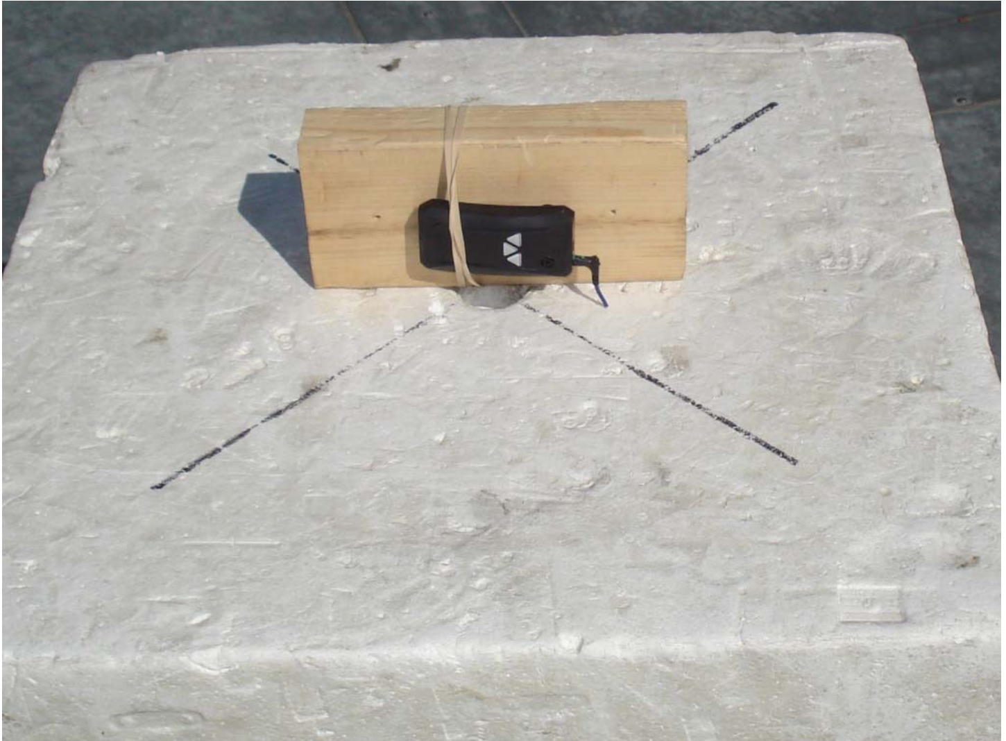
Radiated Emissions – Headset Plug Only
