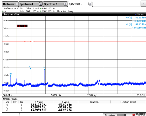
17:51:21 05/04/2018 Figure 7.5.1.2-11: 30 MHz – 25 GHz – BLE – 2440 MHz
