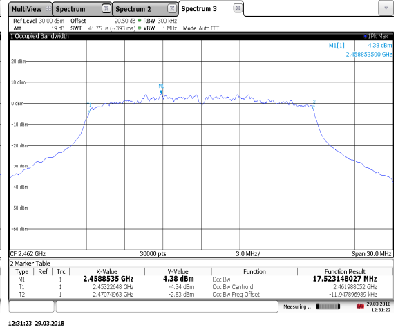
Figure 7.2.2-18: 99% Bandwidth – 802.11n (HT20) – 2462 MHz
