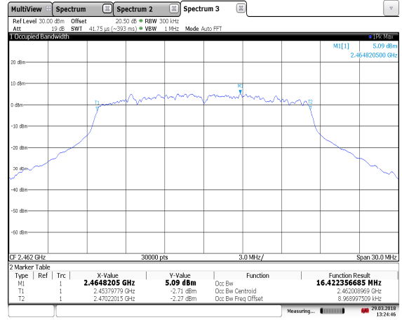
Figure 7.2.2-12: 99% Bandwidth – 802.11g – 2462 MHz
