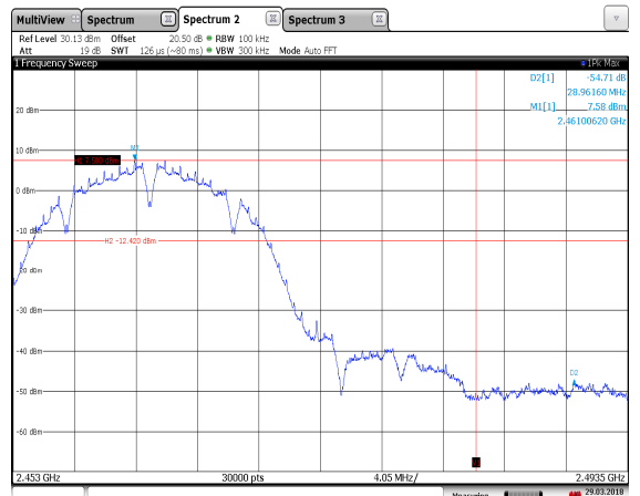
14:50:08 29.03.2018 Figure 7.5.1.2-14: Upper Band-edge – 802.11b – 2462 MHz
