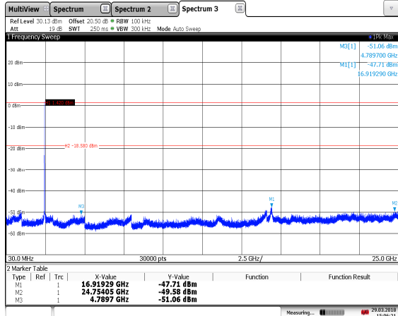
15:06:21 29.03.2018 Figure 7.5.1.2-9: 30 MHz – 25 GHz – 802.11n (HT20) – 2462 MHz
