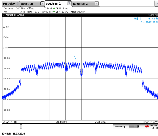
Figure 7.6.2-7: PSD Plot – 802.11n (HT20) – 2412 MHz
