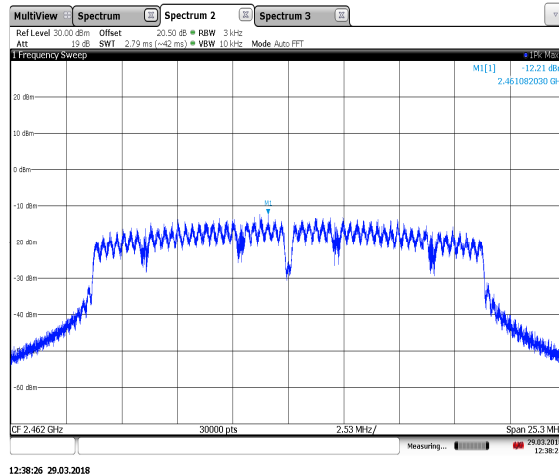
Figure 7.6.2-9: PSD Plot – 802.11n (HT20) – 2462 MHz
