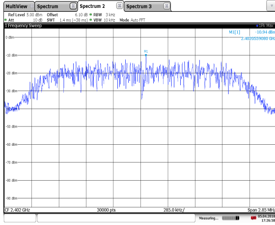
Figure 7.6.2-7: PSD Plot – BLE – 2402 MHz
