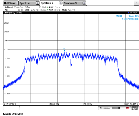
Figure 7.6.2-8: PSD Plot – 802.11n (HT20) – 2437 MHz
