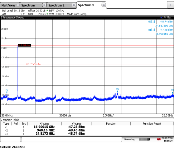
Figure 7.5.1.2-8: 30 MHz – 25 GHz – 802.11n (HT20) – 2437 MHz
