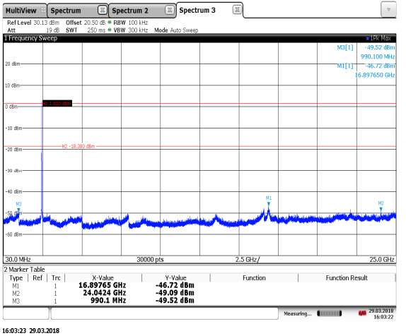
Figure 7.5.1.2-6: 30 MHz – 25 GHz – 802.11g – 2462 MHz
