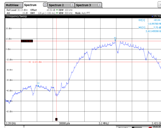
14:13:09 29.03.2018 Figure 7.5.1.2-13: Lower Band-edge – 802.11b – 2412 MHz
