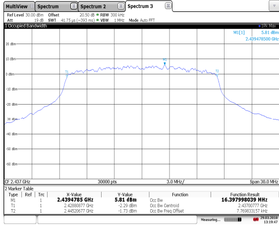
Figure 7.2.2-11: 99% Bandwidth – 802.11g – 2437 MHz
