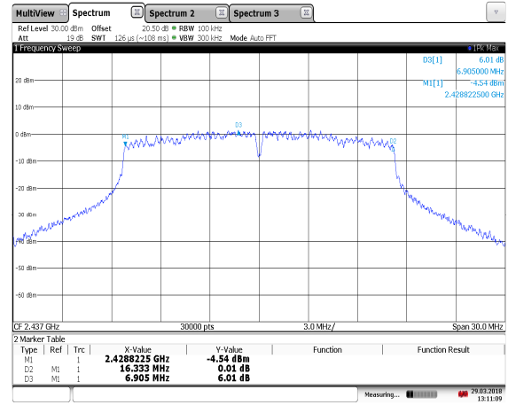
Figure 7.2.2-8: 6dB Bandwidth – 802.11g – 2437 MHz
