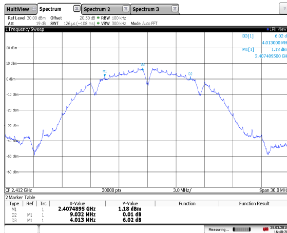
Figure 7.2.2-1: 6dB Bandwidth – 802.11b – 2412 MHz
