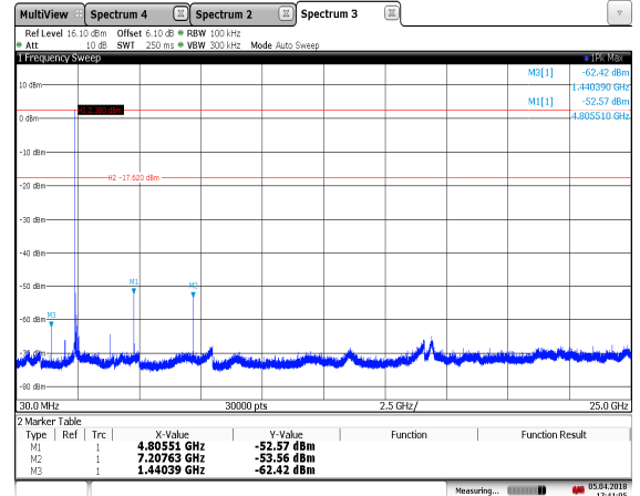
17:41:05 05/04/2018 Figure 7.5.1.2-10: 30 MHz – 25 GHz – BLE – 2402 MHz
