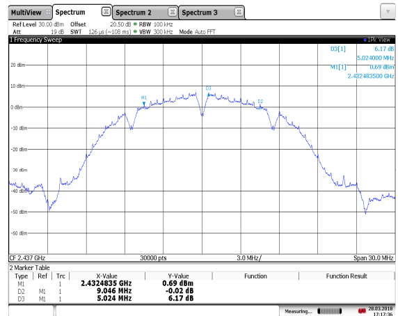
Figure 7.2.2-2: 6dB Bandwidth – 802.11b – 2437 MHz
