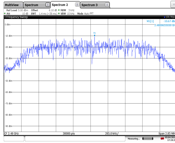
Figure 7.6.2-9: PSD Plot – BLE – 2480 MHz
