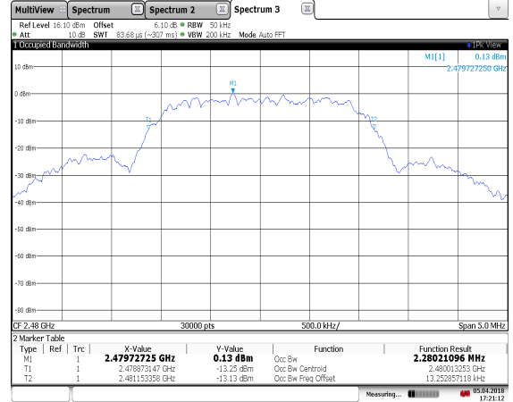
Figure 7.2.2-24: 99% Bandwidth – BLE – 2480 MHz
