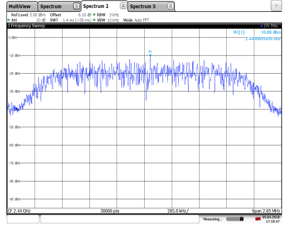
Figure 7.6.2-8: PSD Plot – BLE – 2440 MHz
