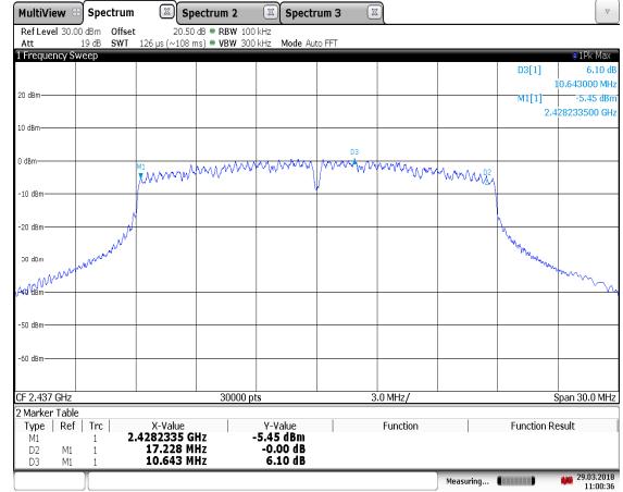
11:00:37 29.03.2018 Figure 7.2.2-14: 6dB Bandwidth – 802.11n (HT20) – 2437 MHz
