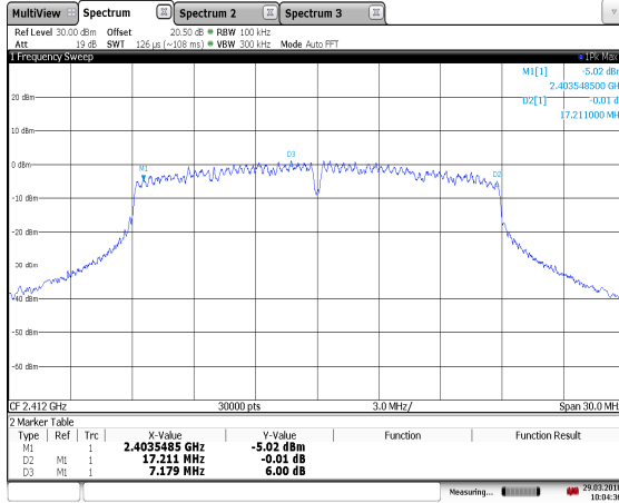
10:04:36 29.03.2018 Figure 7.2.2-13: 6dB Bandwidth – 802.11n (HT20) – 2412 MHz
