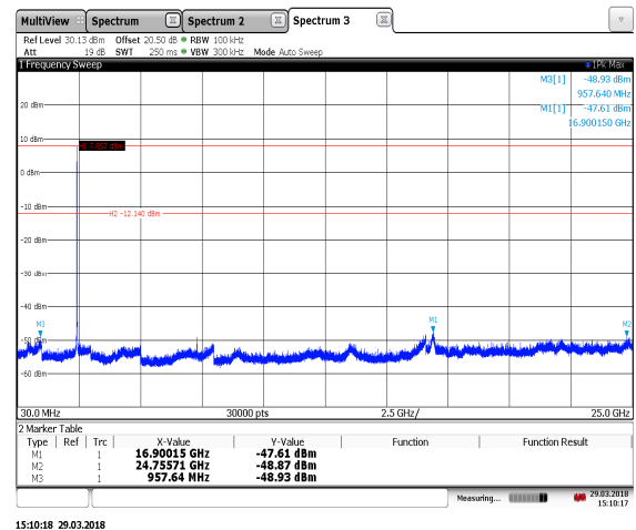
Figure 7.5.1.2-2: 30 MHz – 25 GHz – 802.11b – 2437 MHz
