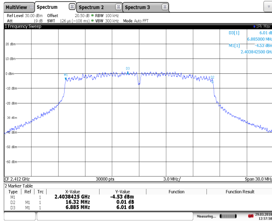
Figure 7.2.2-7: 6dB Bandwidth – 802.11g – 2412 MHz
