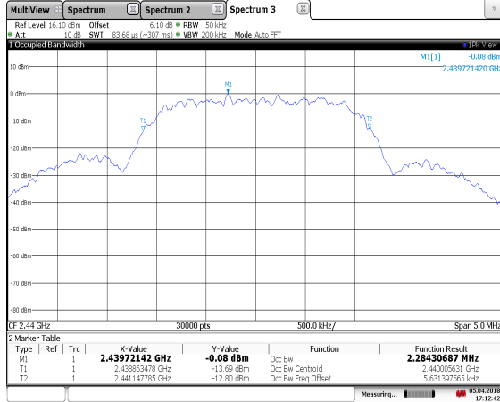
Figure 7.2.2-23: 99% Bandwidth – BLE – 2440 MHz
