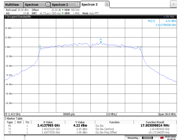
10:48:57 29.03.2018 Figure 7.2.2-16: 99% Bandwidth – 802.11n (HT20) – 2412 MHz
