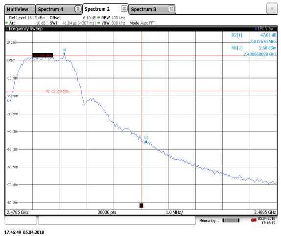
Figure 7.5.1.2-20: Upper Band-edge – BLE – 2480 MHz
