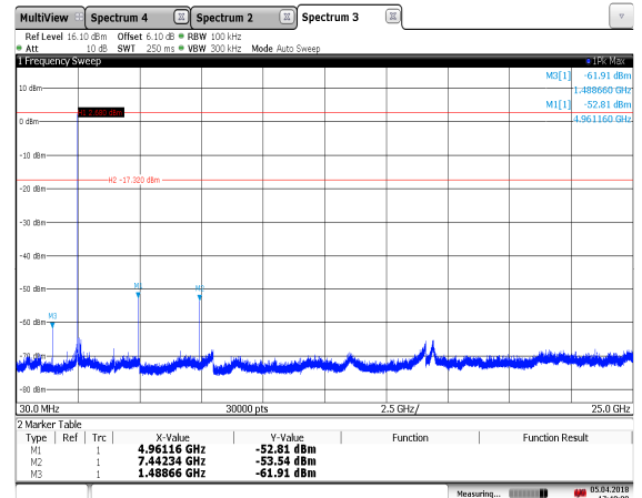
17:48:10 05/04/2018 Figure 7.5.1.2-12: 30 MHz – 25 GHz – BLE – 2480 MHz
