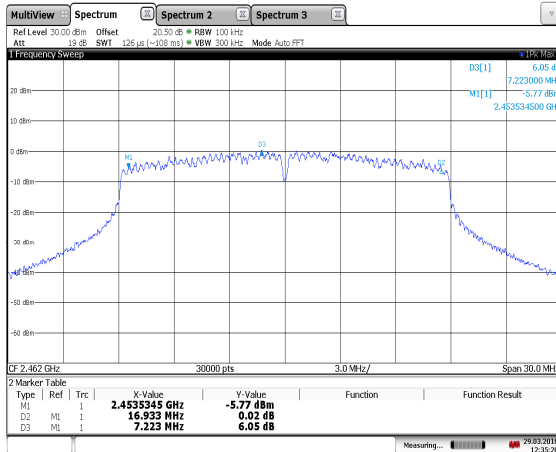
12:35:20 29.03.2018 Figure 7.2.2-15: 6dB Bandwidth – 802.11n (HT20) – 2462 MHz
