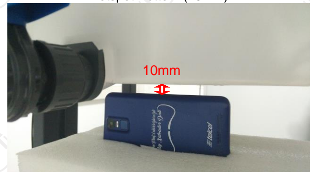
Hotspot Left (10mm)
