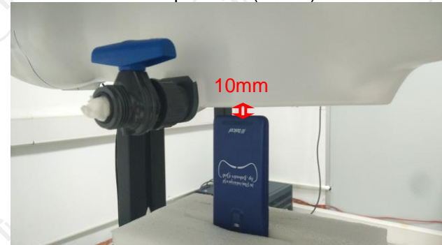
Hotspot Bottom (10mm)
