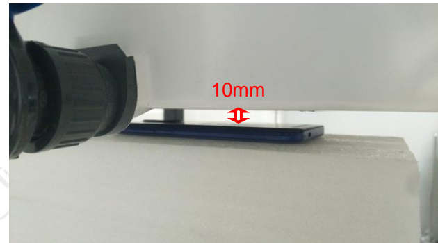
Body worn – Back (10mm)
