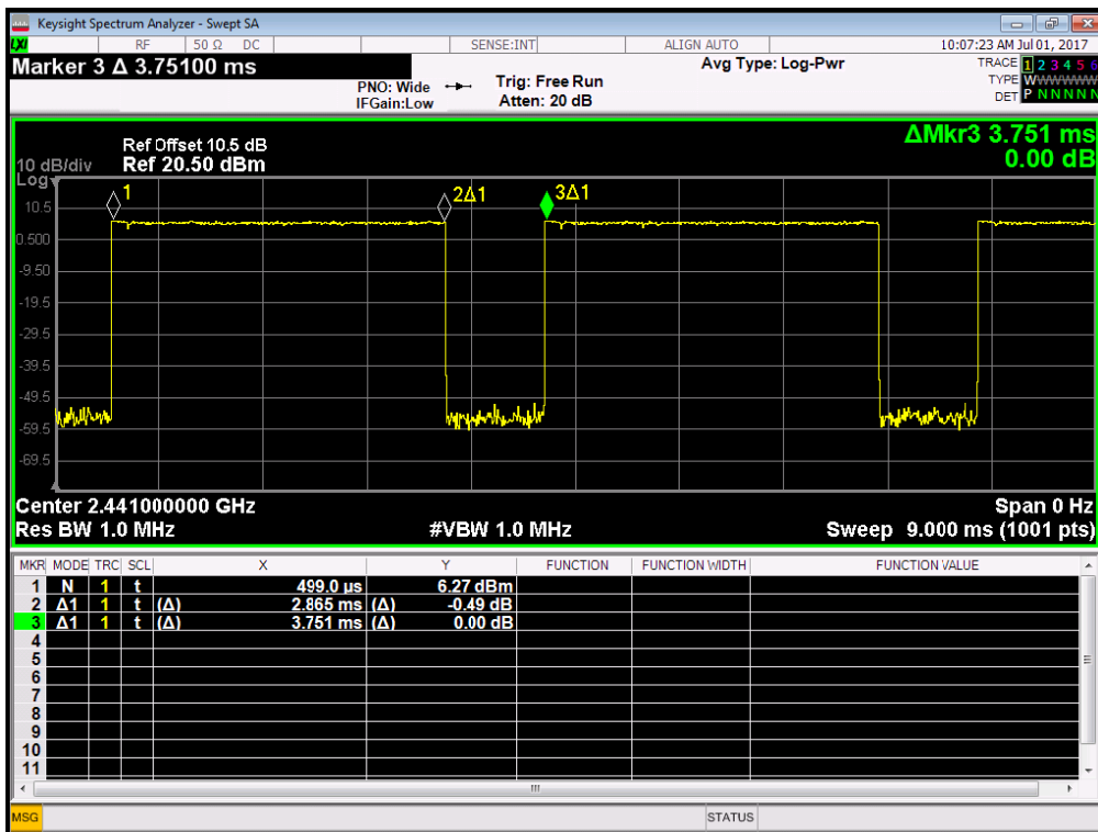
39 Channel @ 2DH5
