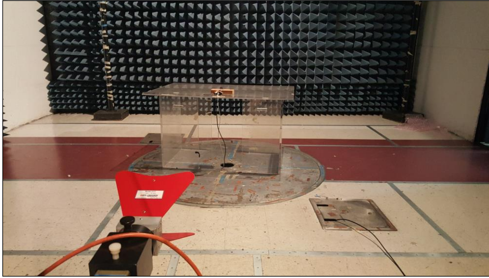
Photograph 3. Radiated Spurious Emissions, Test Setup (2)
