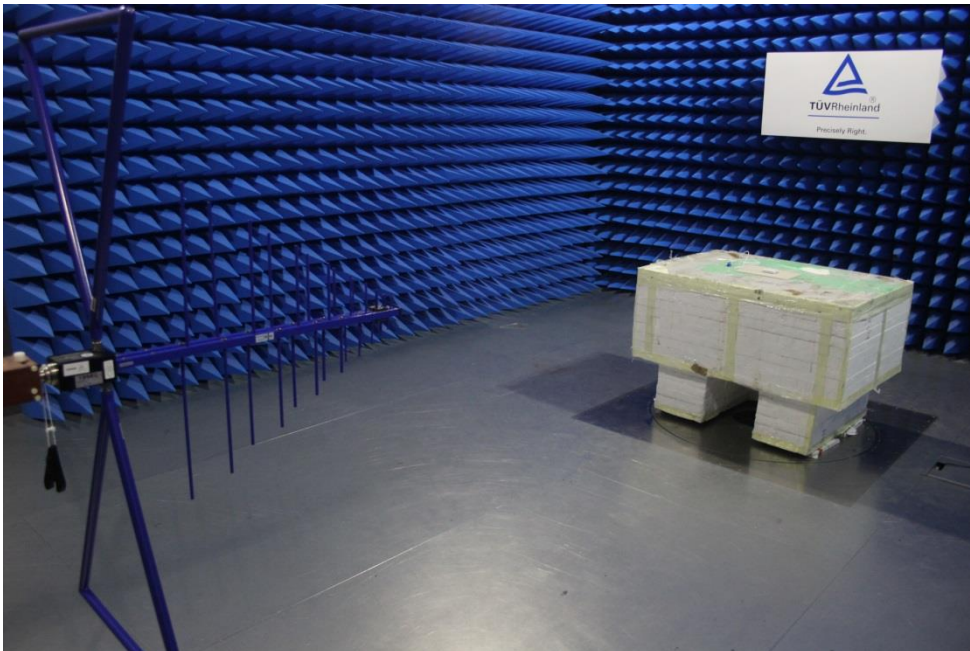
Radiated emissions setup below 1 GHz
