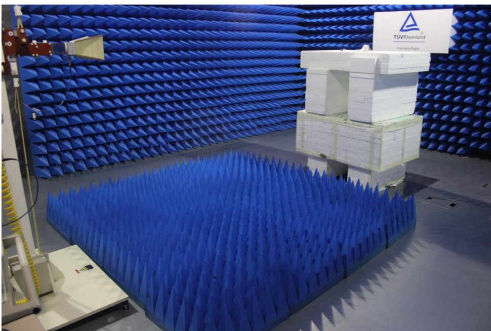
Radiated emissions setup above 1 GHz
