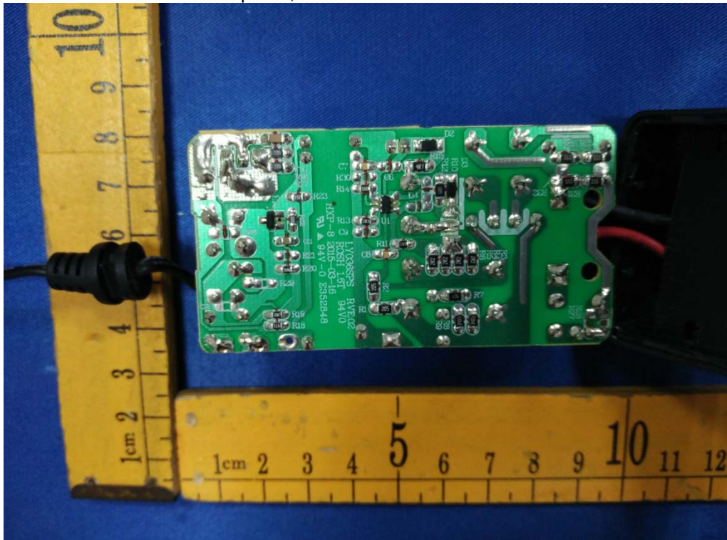
Adapter 3, M/N: LY036SPS-120300U
