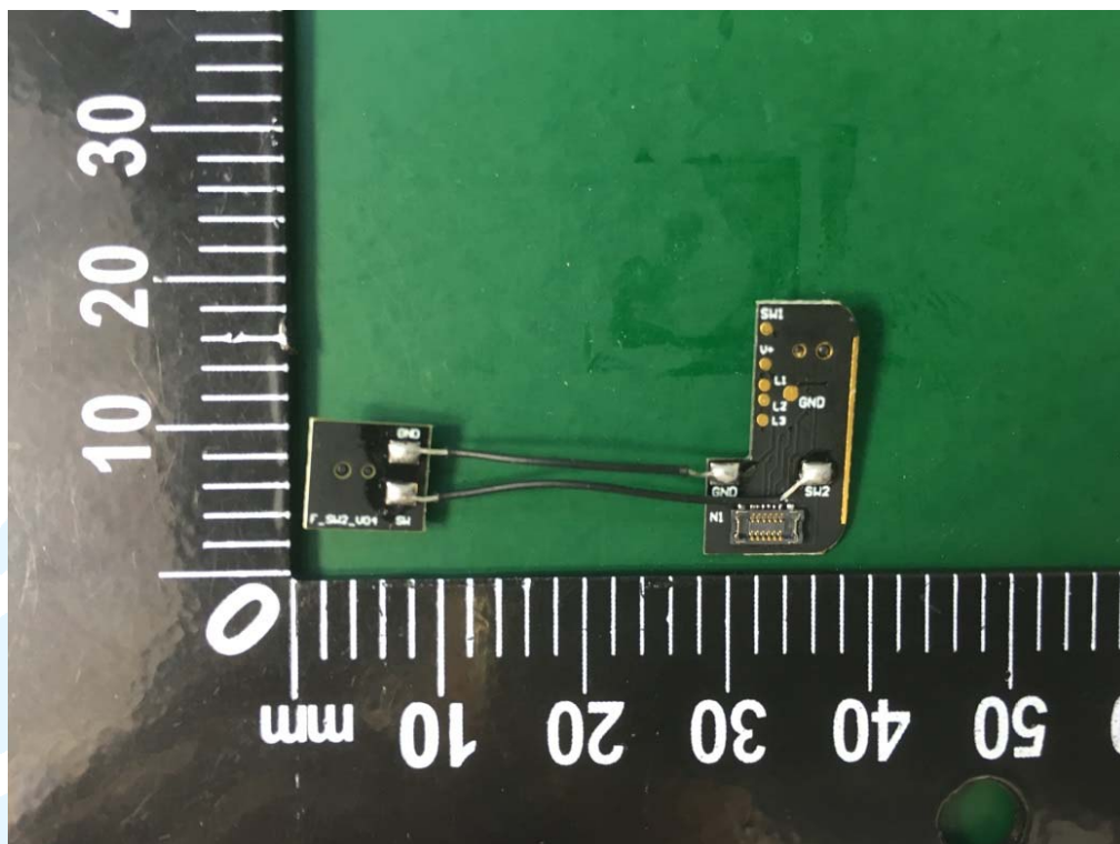
EUT Photo #13 PCB View
