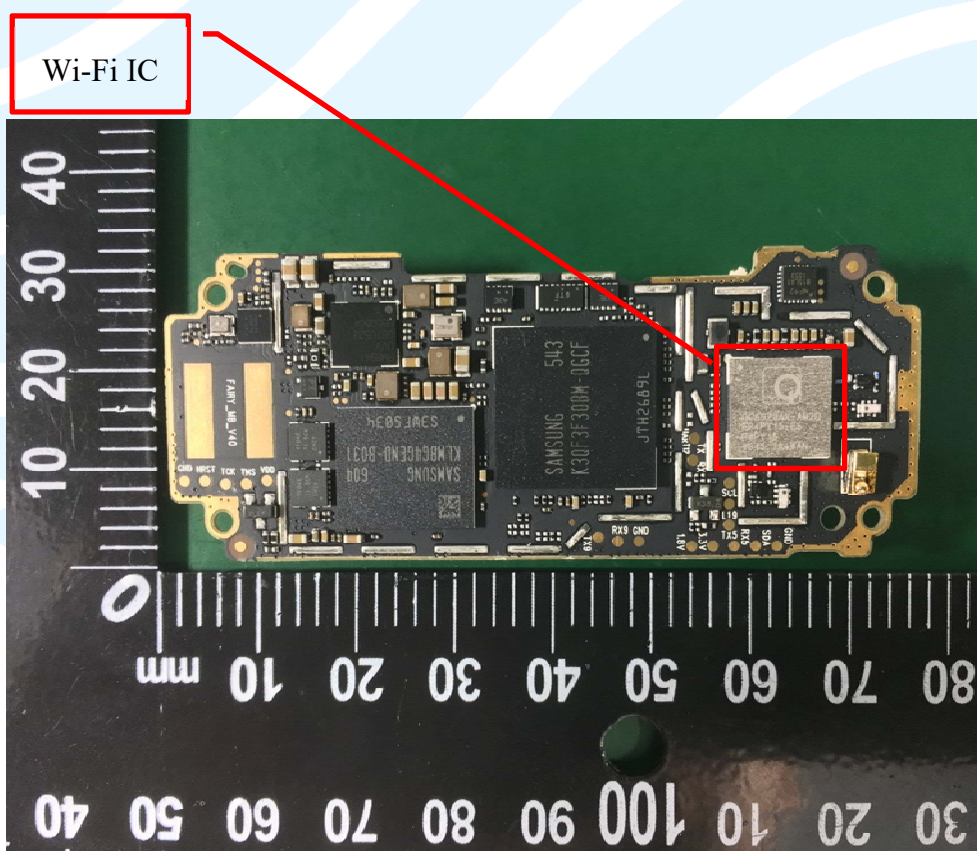
EUT Photo #12 PCB View
