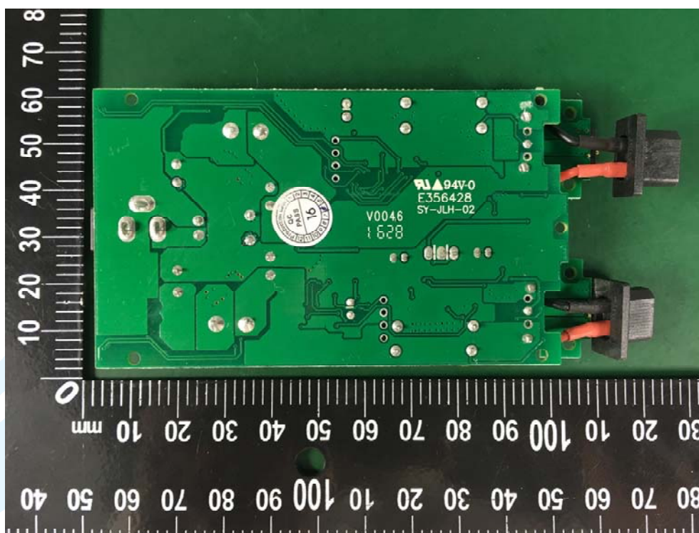
EUT (Charging Dock) Photo #17 PCB View
