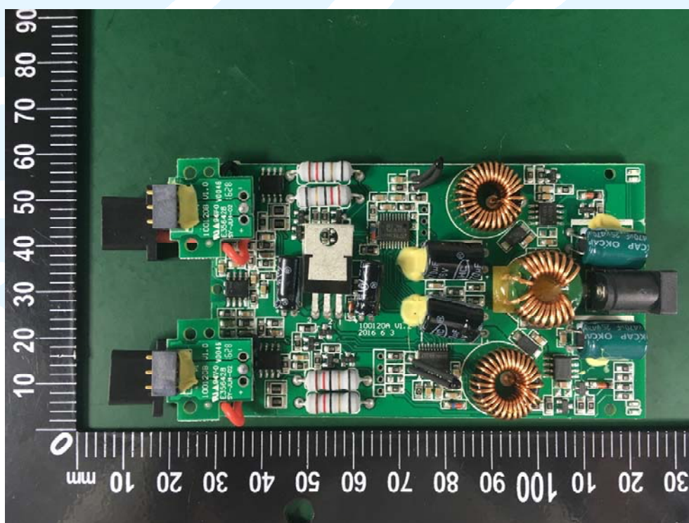
EUT (Charging Dock) Photo #16 PCB View
