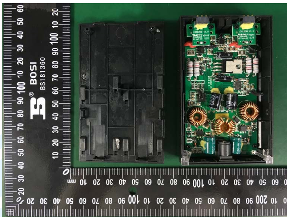
EUT (Charging Dock) Photo #15 Uncover View
