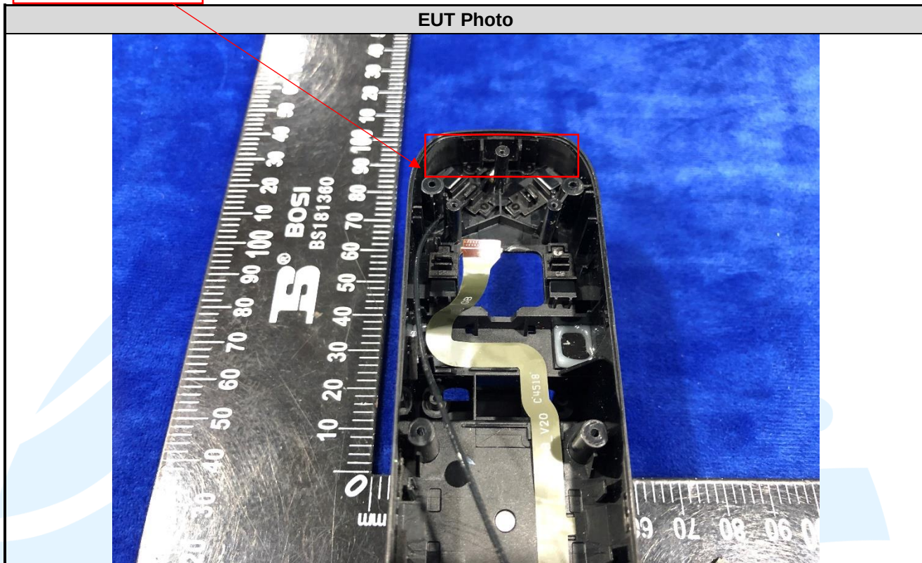
RF Antenna 2
