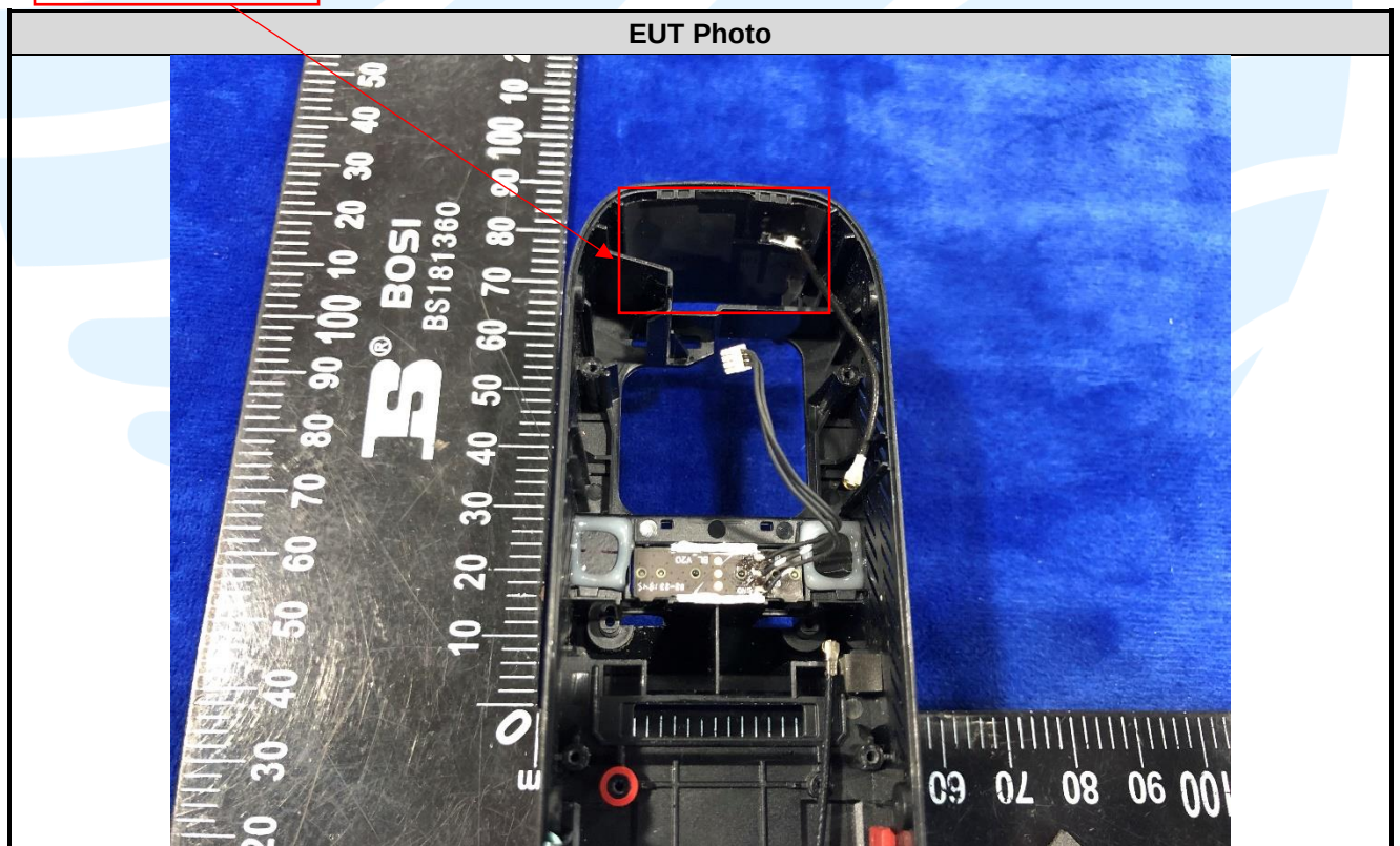
RF Antenna 1
