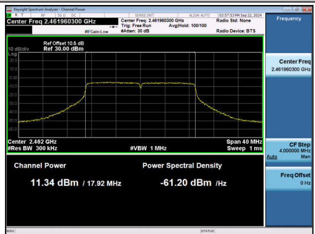
11N20MIMO-Ant2-2462-PASS
