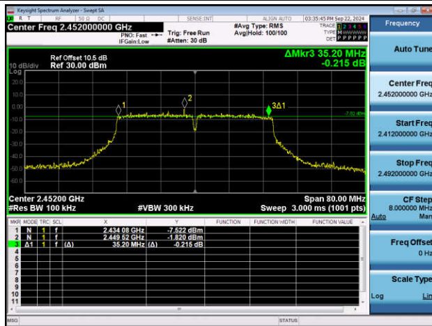
11N40MIMO-Ant1-2452-PASS
