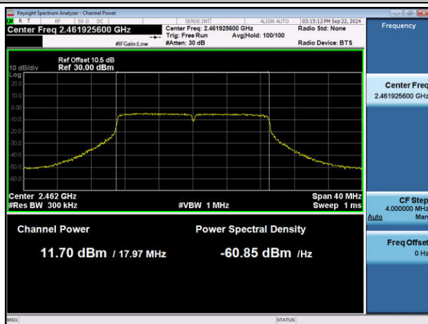
11N20MIMO-Ant1-2462-PASS
