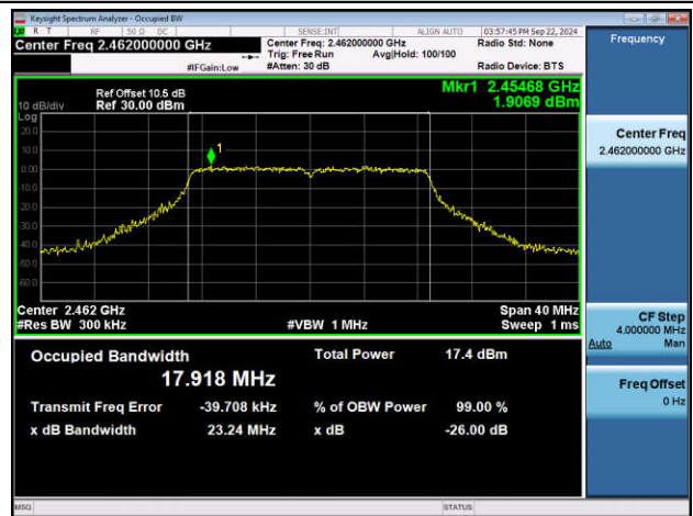
11N20MIMO-Ant2-2462
