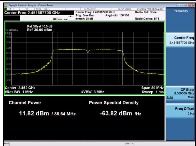
11N40MIMO-Ant2-2452-PASS
