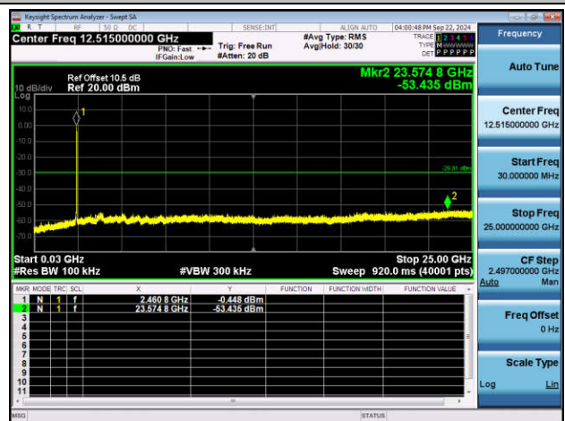
11N20MIMO-Ant2-2462-30~25000-PASS
