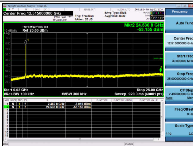
11N20MIMO-Ant1-2462-30~25000-PASS
