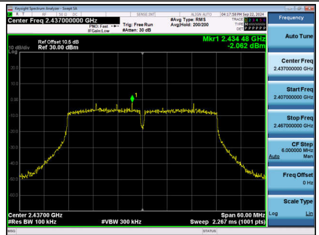
11N40MIMO-Ant2-2437-0~Reference-PASS
