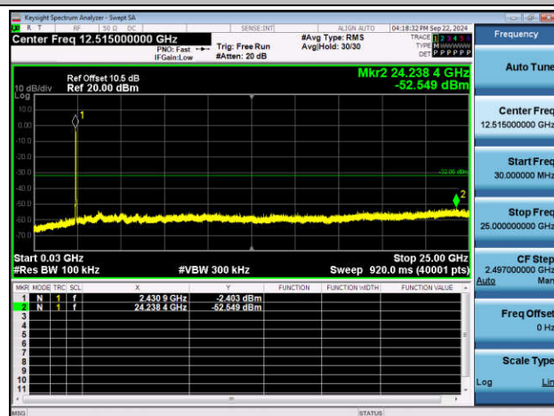
11N40MIMO-Ant2-2452-0~Reference-PASS
