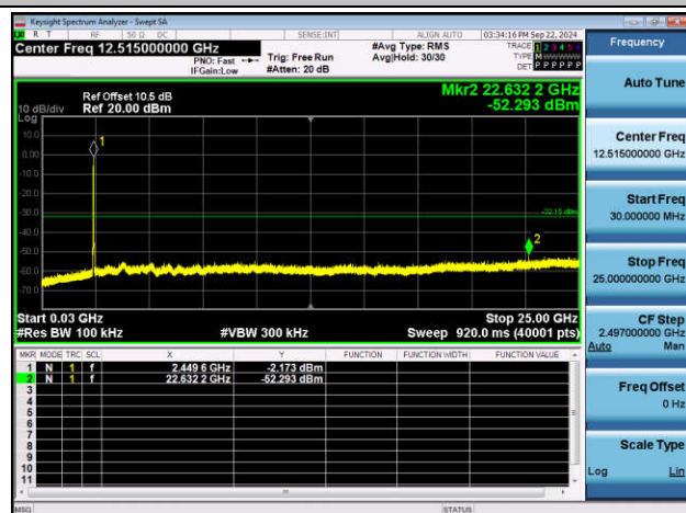
11N40MIMO-Ant1-2452-0~Reference-PASS
