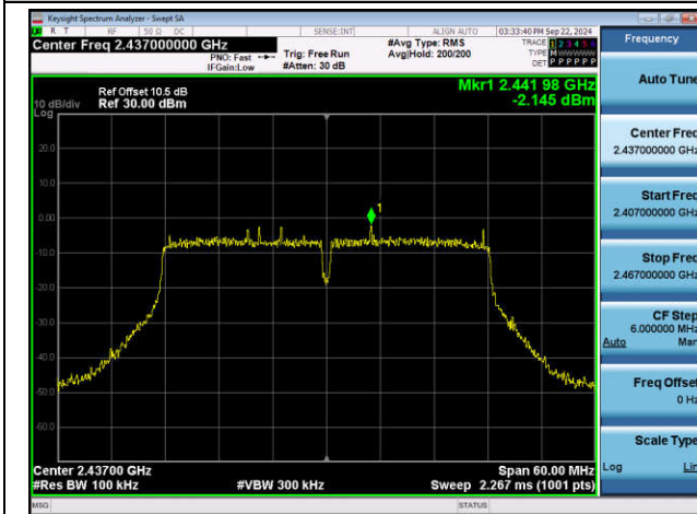
11N40MIMO-Ant1-2437-0~Reference-PASS
