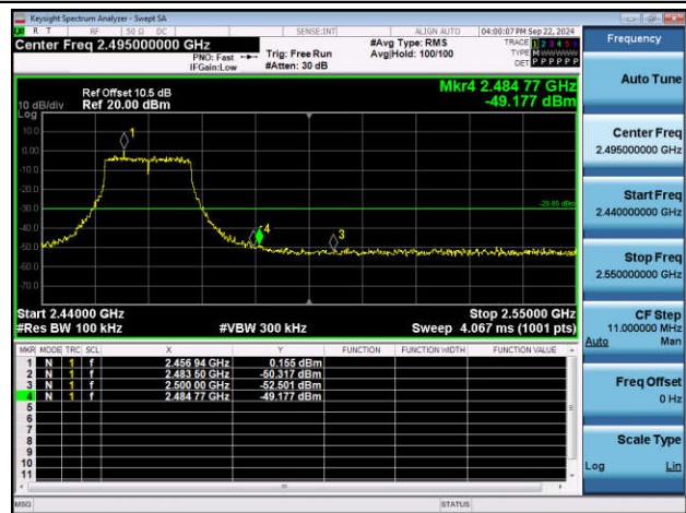
11N20MIMO-Ant2-2462-PASS
